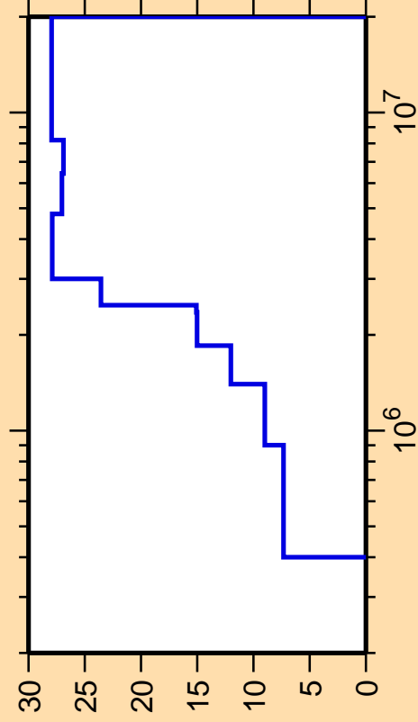
\Delta\sigma/\sigma vs. E for ^{114}\text{Cd}(n,n_1)
