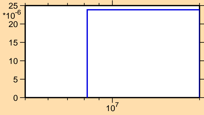
\sigma vs. E for ^{114}\text{Cd}(n,n\alpha)
