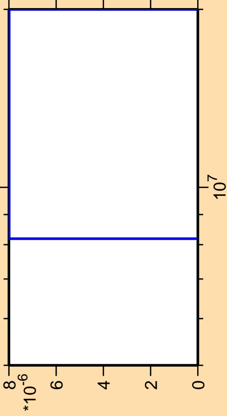
\Delta\sigma/\sigma vs. E for ^{114}\text{Cd}(n,2np)
