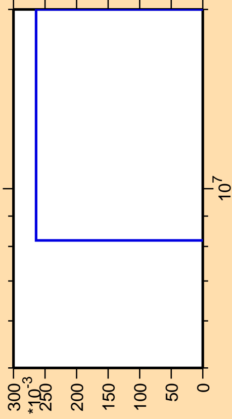
\Delta\sigma/\sigma vs. E for ^{114}\text{Cd}(n,2n\alpha)
