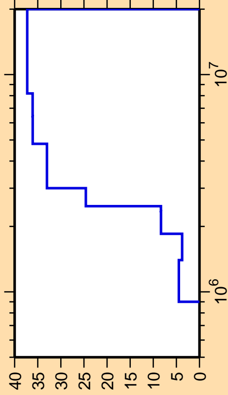
\Delta\sigma/\sigma vs. E for ^{114}\text{Cd}(n,n_2)
