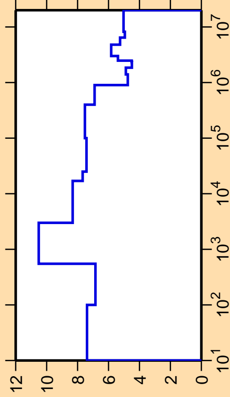
\Delta\sigma/\sigma vs. E for ^{114}\text{Cd}(n,\text{nonel.})
