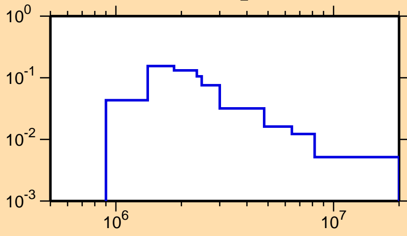
\sigma vs. E for ^{114}\text{Cd}(n,n_2)
