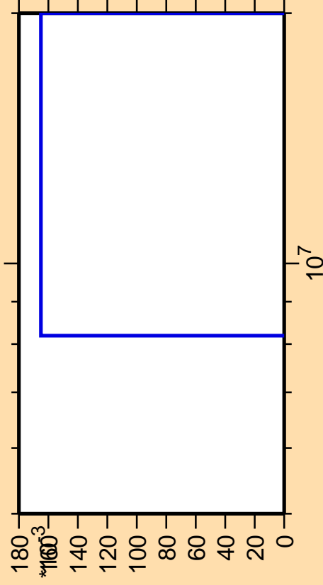
\Delta\sigma/\sigma vs. E for ^{114}\text{Cd}(n,nt)
