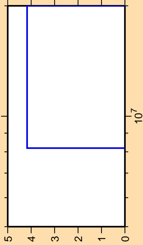
\Delta\sigma/\sigma vs. E for ^{114}\text{Cd}(n,\text{nd})
