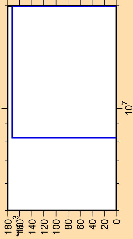
\Delta\sigma/\sigma vs. E for ^{114}\text{Cd}(n,\text{He}3)
