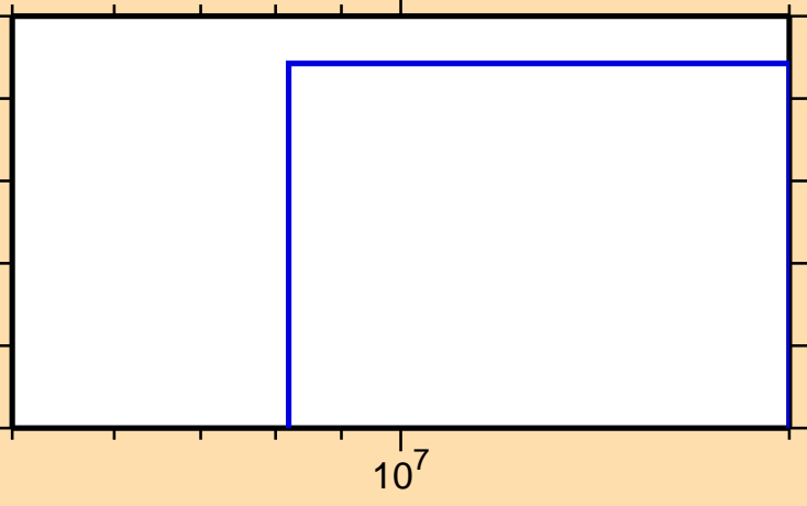
\sigma vs. E for ^{115}\text{Cd}(n,3n)
