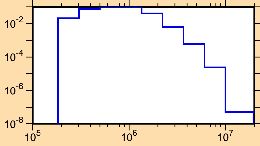
\sigma vs. E for ^{115}\text{Cd}(n,n_4)
