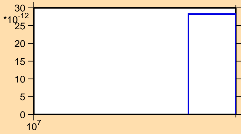
\sigma vs. E for ^{116}\text{Cd}(n,\text{nd})
