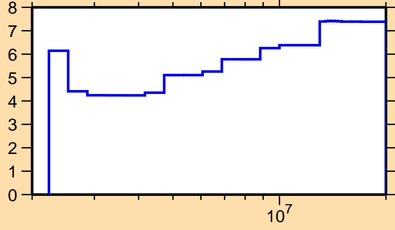
\Delta\sigma/\sigma vs. E for ^{116}\text{Cd}(n,n\text{onel.})
