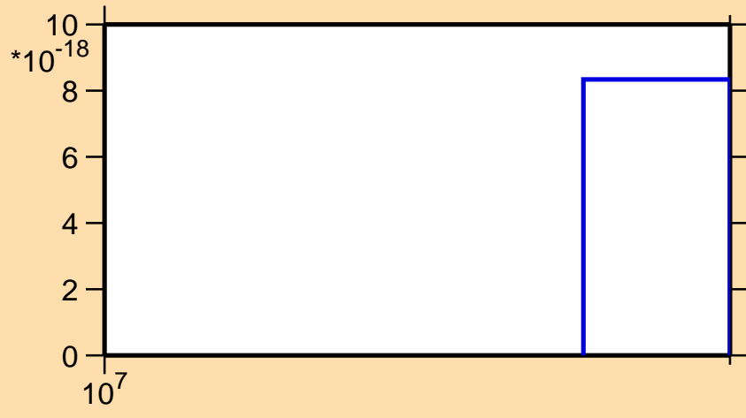
\sigma vs. E for ^{116}\text{Cd}(n,2np)
