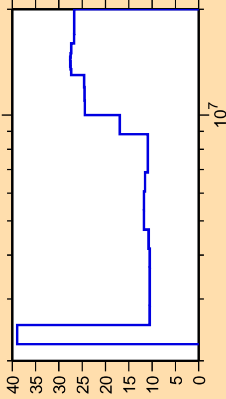
\Delta\sigma/\sigma vs. E for ^{116}\text{Cd}(n,n\text{cont.})
