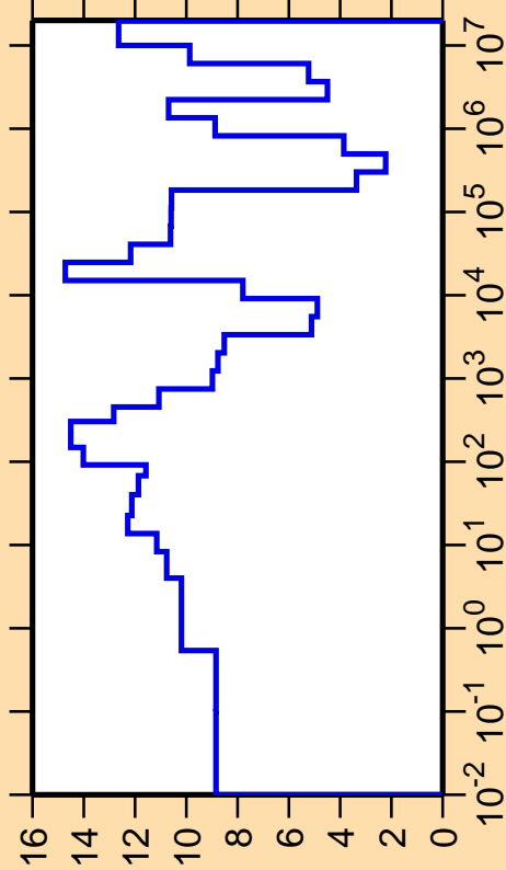
\Delta\sigma/\sigma vs. E for ^{116}\text{Cd}(n,\text{el.})
