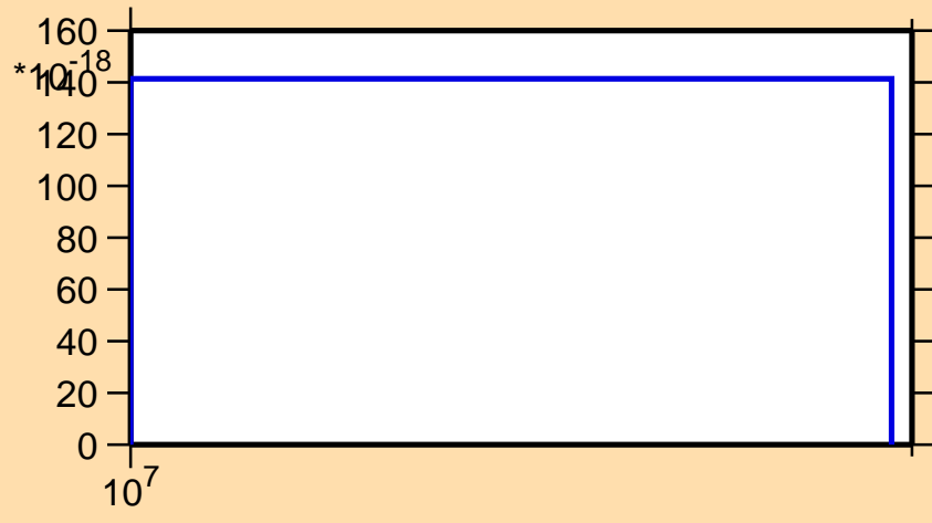
\sigma vs. E for ^{116}\text{Cd}(n,\text{He}3)
