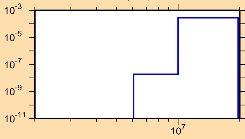
\sigma vs. E for ^{116}\text{Cd}(n,\alpha)
