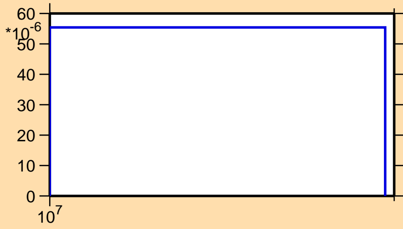
\sigma vs. E for ^{116}\text{Cd}(n,np)
