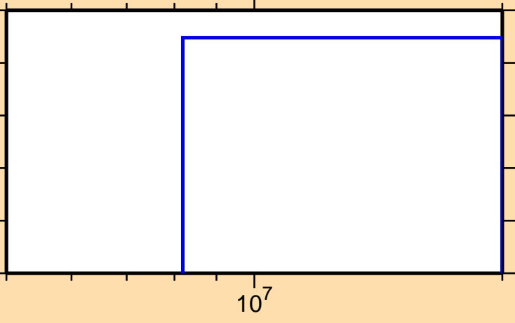
\sigma vs. E for ^{116}\text{Cd}(n,3n)
