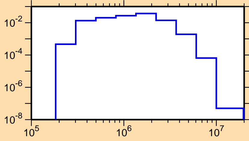
\sigma vs. E for ^{117}\text{Cd}(n,n_3)
