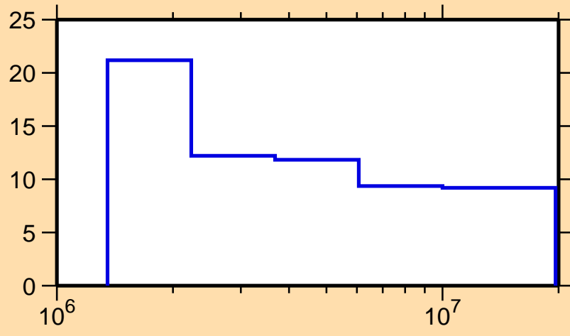
\Delta\sigma/\sigma vs. E for ^{117}\text{Cd}(n,n\text{onel.})
