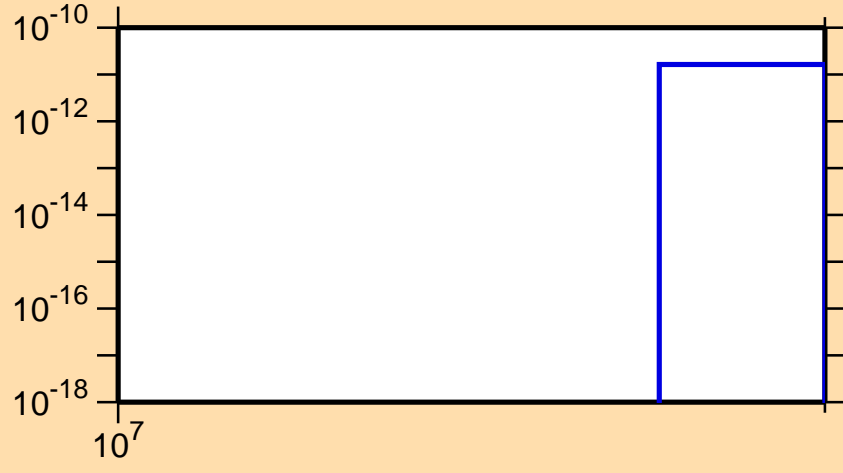
\sigma vs. E for ^{117}\text{Cd}(n,nt)
