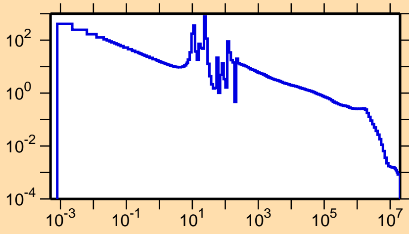
\sigma vs. E for ^{117}\text{Cd}(n,\gamma)
