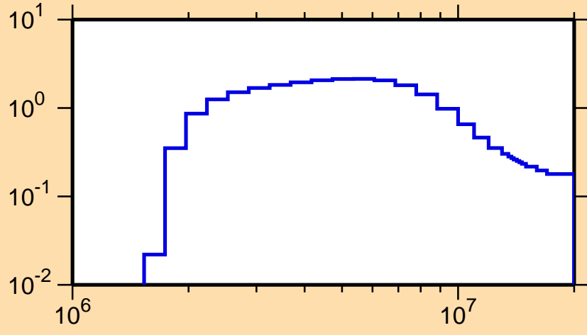
\sigma vs. E for ^{117}\text{Cd}(n,n\text{cont.})
