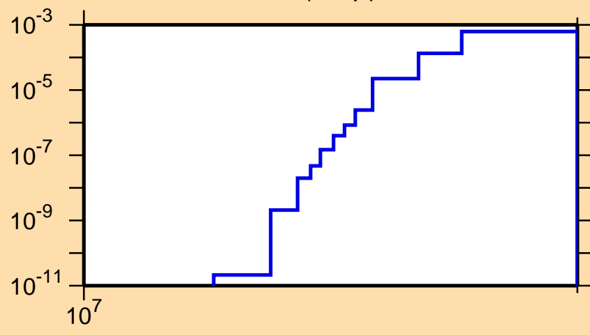
\sigma vs. E for ^{117}\text{Cd}(n,np)
