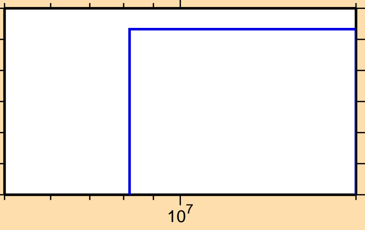
\sigma vs. E for ^{117}\text{Cd}(n,d)
