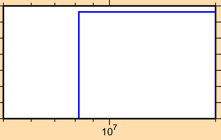
\sigma vs. E for ^{117}\text{Cd}(n,np)
