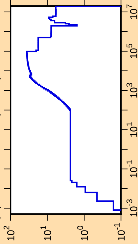
\Delta\mu/\mu vs. E for ^{119}\text{Cd}(\text{mt251})
