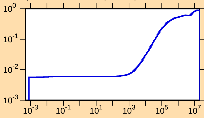
\mu vs. E for ^{119}\text{Cd}(\text{mt251})
