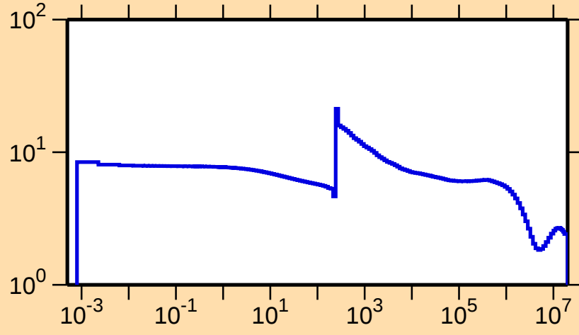
\sigma vs. E for ^{119}\text{Cd}(n,\text{el.})
