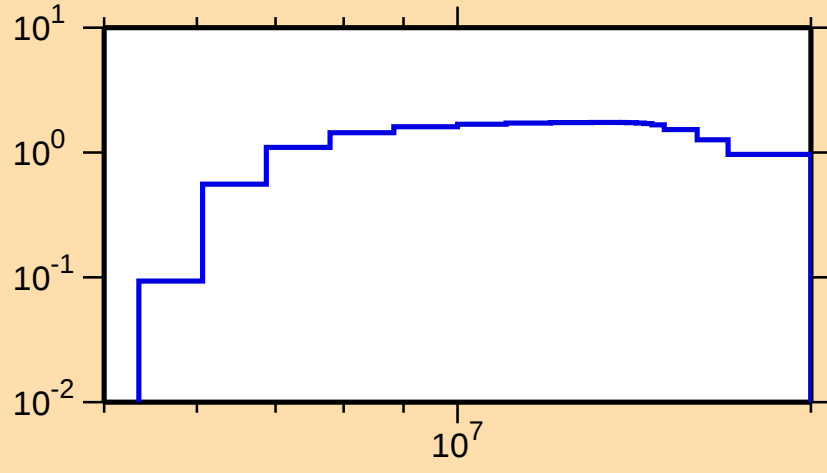
\sigma vs. E for ^{119}\text{Cd}(n,2n)
