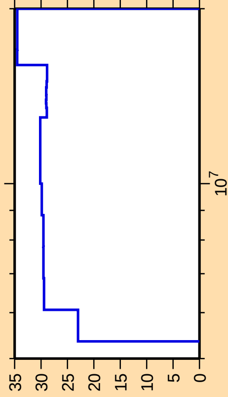
\Delta\sigma/\sigma vs. E for ^{119}\text{Cd}(n,n_1)
