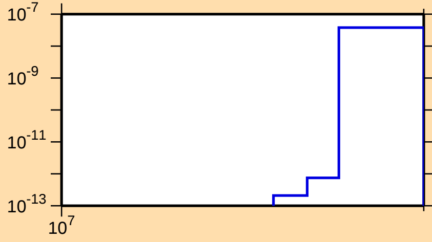
\sigma vs. E for ^{119}\text{Cd}(n,\text{nd})
