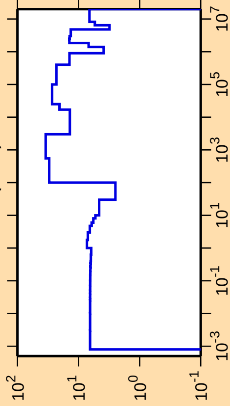
\Delta\sigma/\sigma vs. E for ^{119}\text{Cd}(n,\text{el.})
