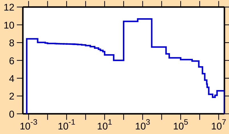
\sigma vs. E for ^{119}\text{Cd}(n,\text{el.})
