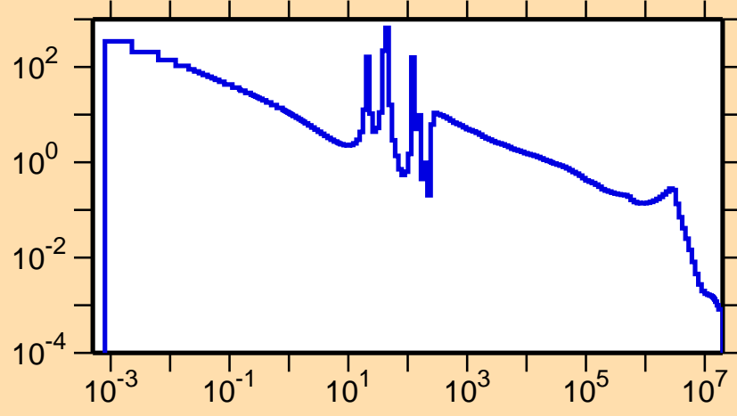
\sigma vs. E for ^{119}\text{Cd}(n,\gamma)
