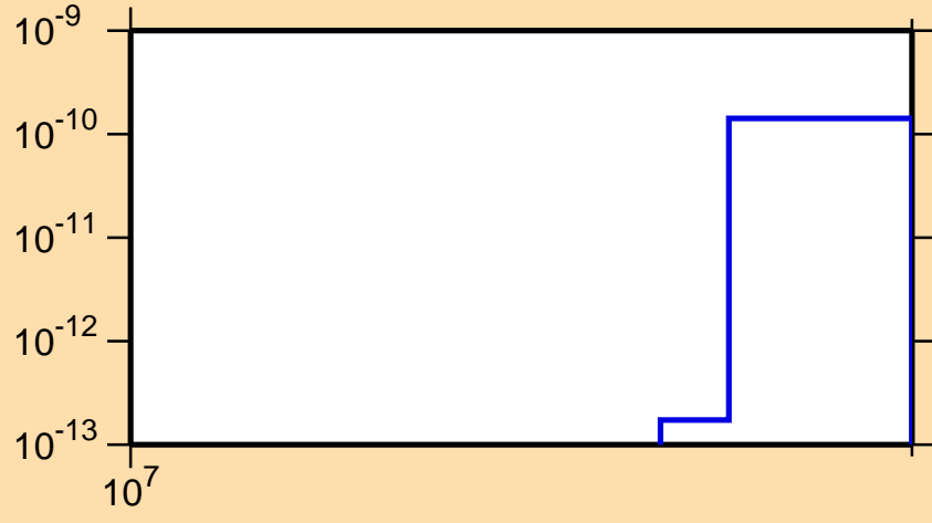
\sigma vs. E for ^{119}\text{Cd}(n,2n\alpha)
