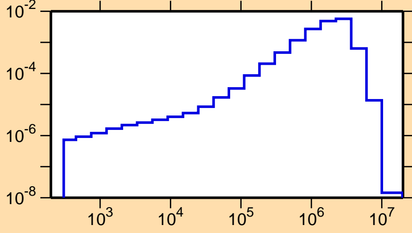
\sigma vs. E for ^{119}\text{Cd}(n,n_1)
