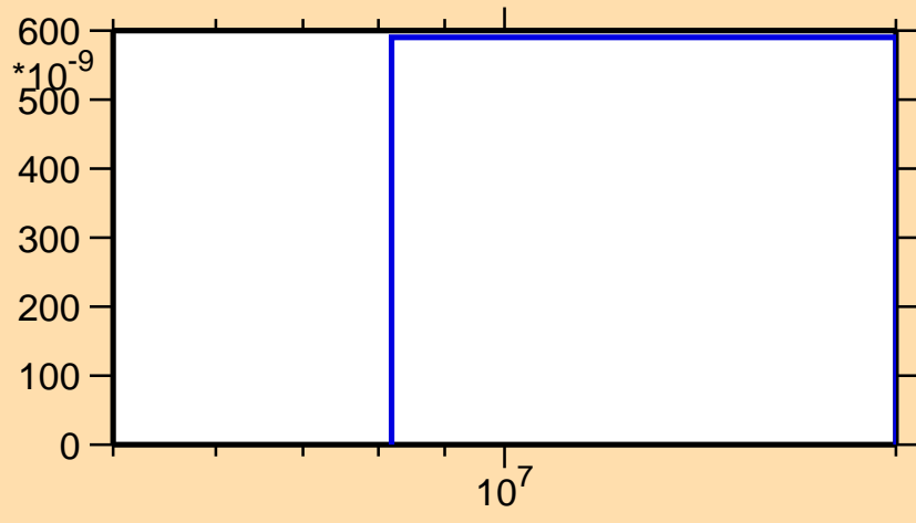
\sigma vs. E for ^{119}\text{Cd}(n,n\alpha)
