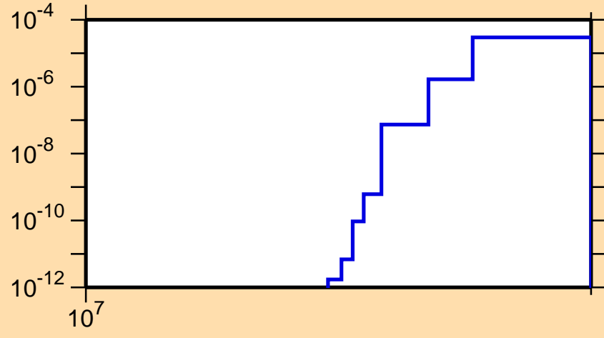
\sigma vs. E for ^{120}\text{Cd}(n,np)
