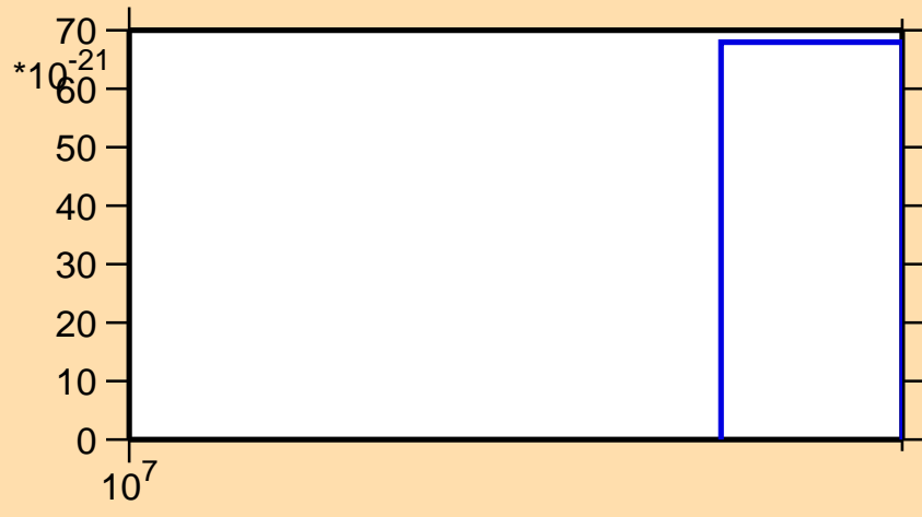
\sigma vs. E for ^{120}\text{Cd}(n,2np)
