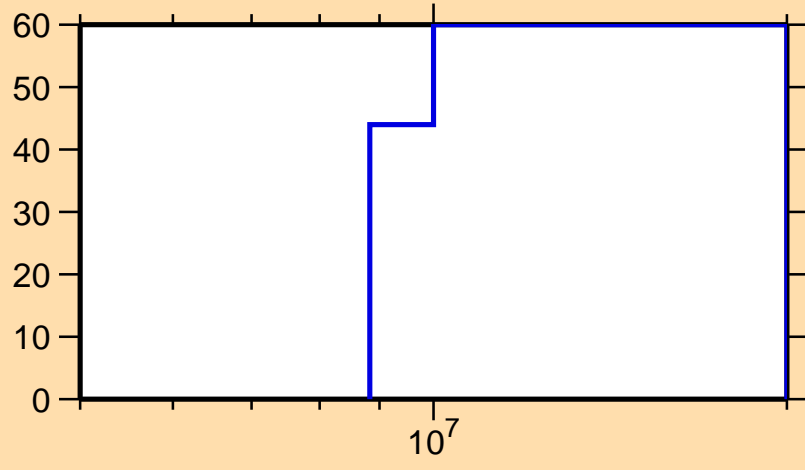
\Delta\sigma/\sigma vs. E for ^{120}\text{Cd}(n,ncont.)
