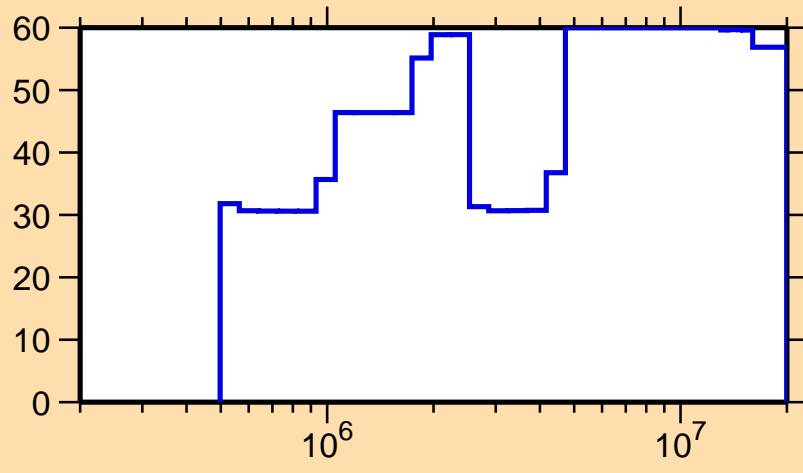
\Delta\sigma/\sigma vs. E for ^{120}\text{Cd}(n,n_1)
