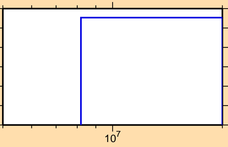
\sigma vs. E for ^{120}\text{Cd}(n,2np)
