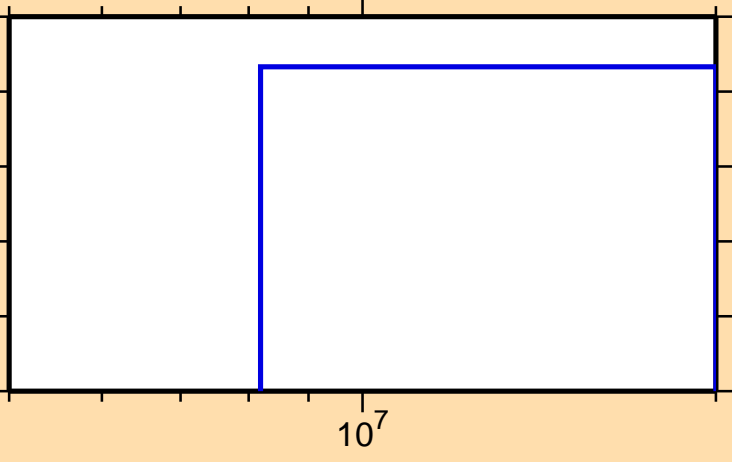
\sigma vs. E for ^{120}\text{Cd}(n,n\alpha)
