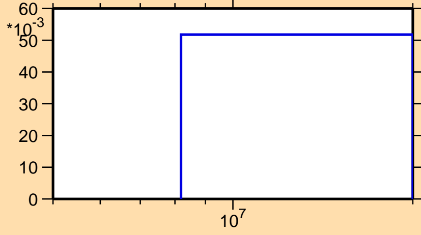
\sigma vs. E for ^{120}\text{Cd}(n,3n)
