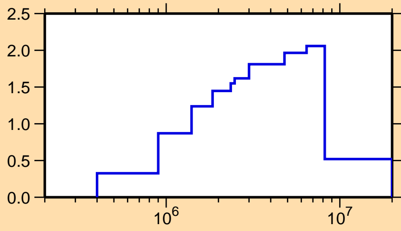
\sigma vs. E for ^{120}\text{Cd}(n,\text{inel.})
