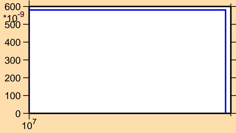
\sigma vs. E for ^{122}\text{Cd}(n,d)
