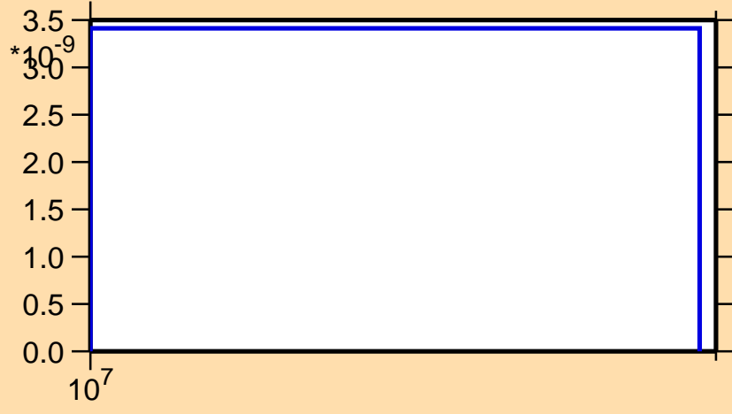
\sigma vs. E for ^{122}\text{Cd}(n,n\alpha)
