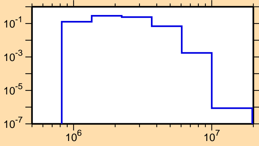
\sigma vs. E for ^{122}\text{Cd}(n,n_2)
