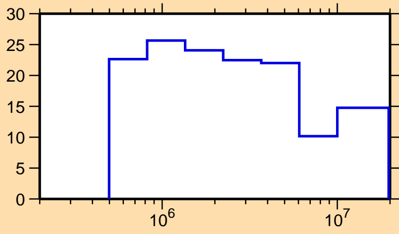
\Delta\sigma/\sigma vs. E for ^{122}\text{Cd}(n,\text{tot.})
