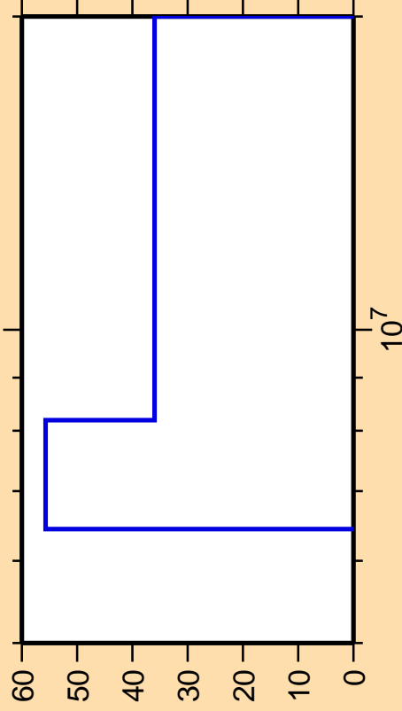
\Delta\sigma/\sigma vs. E for ^{122}\text{Cd}(n,2n)
