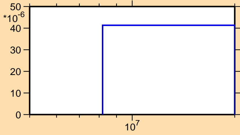
\sigma vs. E for ^{122}\text{Cd}(n,p)
