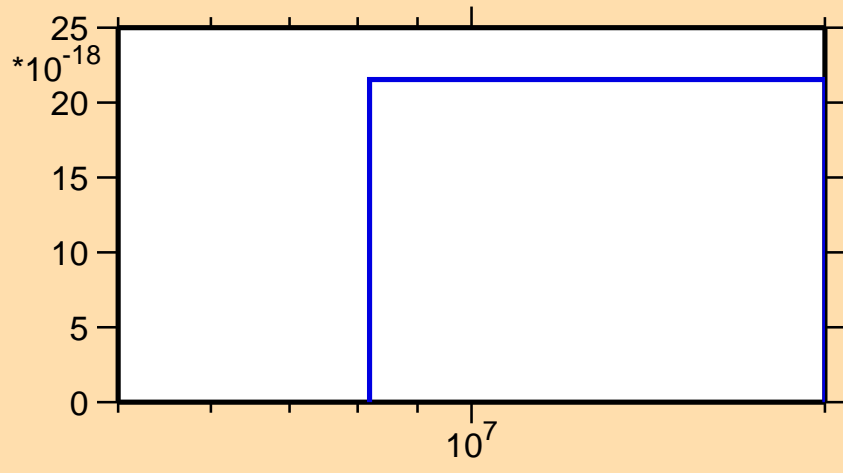
\sigma vs. E for ^{122}\text{Cd}(n,\text{nd})
