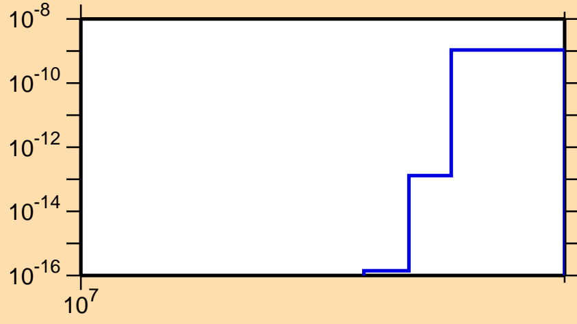
\sigma vs. E for ^{123}\text{Cd}(n,\text{nd})
