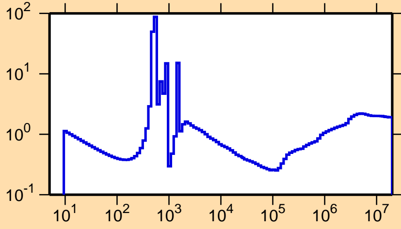
\sigma vs. E for ^{123}\text{Cd}(n,\text{nonel.})
