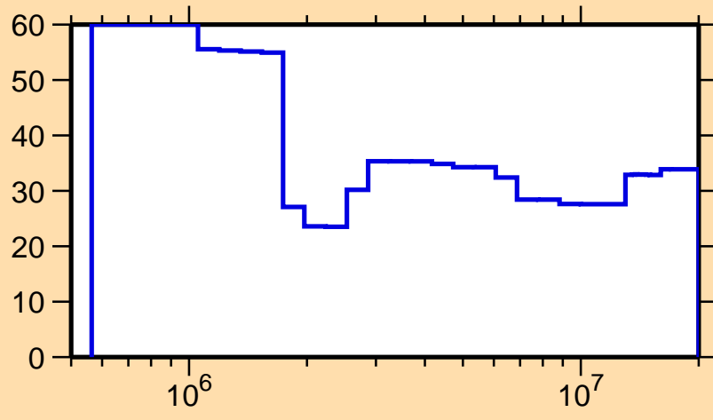
\Delta\sigma/\sigma vs. E for ^{124}\text{Cd}(n,\text{nonel.})
