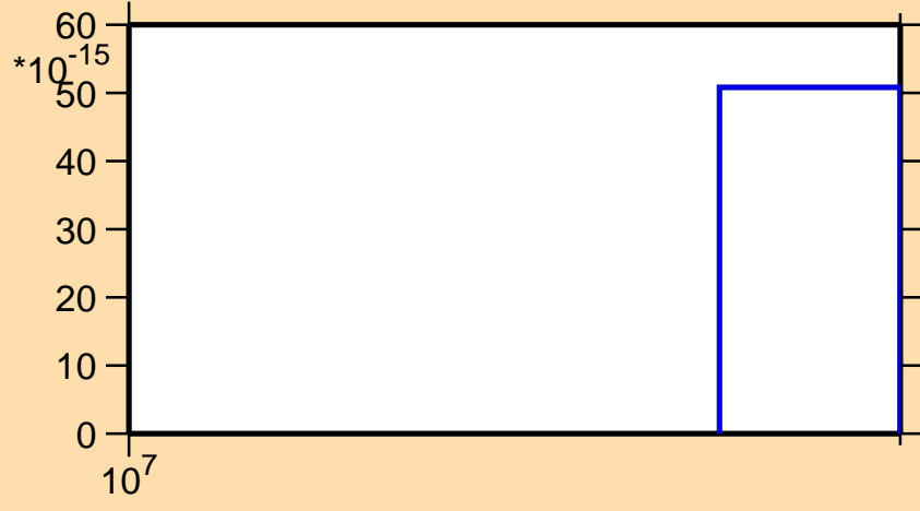
\sigma vs. E for ^{124}\text{Cd}(n,nt)
