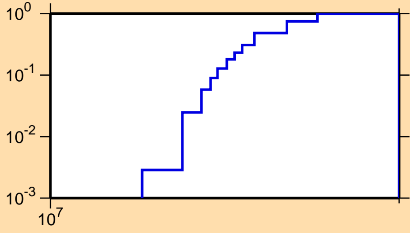
\sigma vs. E for ^{124}\text{Cd}(n,3n)
