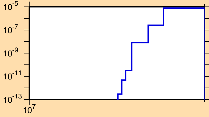
\sigma vs. E for ^{124}\text{Cd}(n,d)
