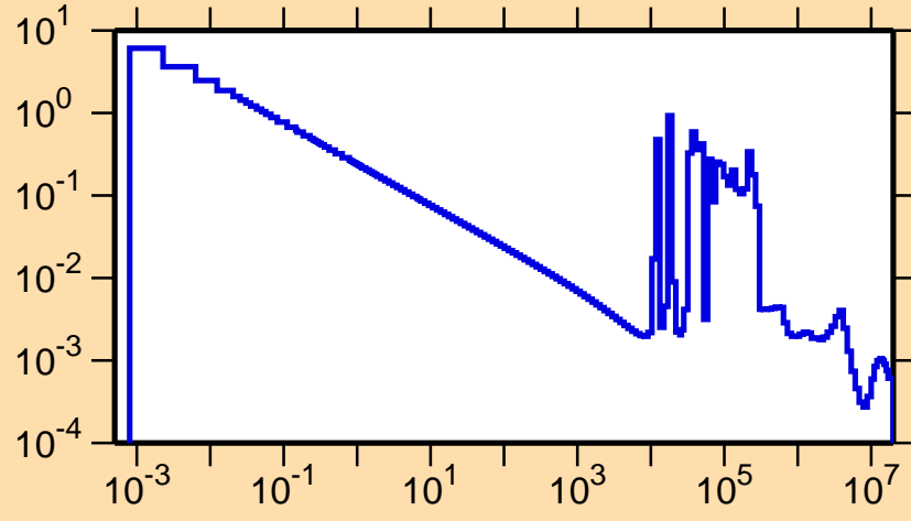
\sigma vs. E for ^{124}\text{Cd}(n,\gamma)
