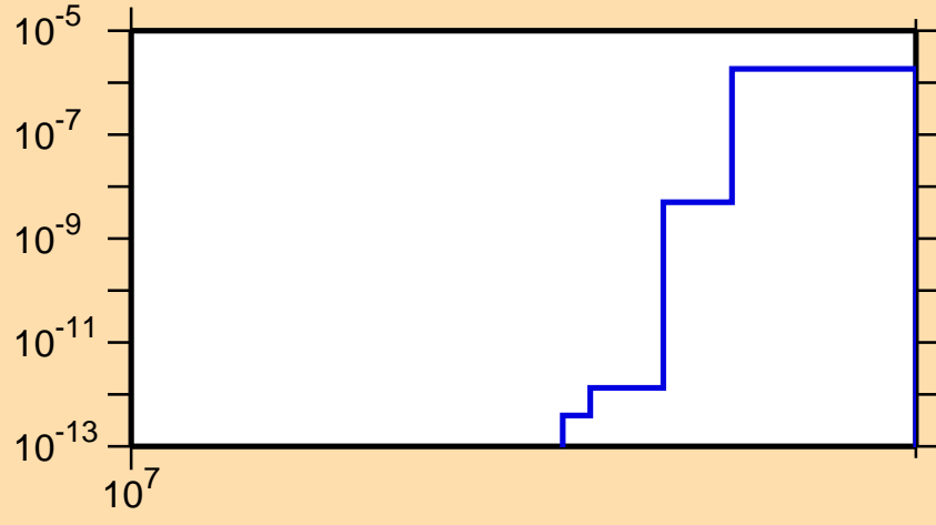
\sigma vs. E for ^{124}\text{Cd}(n,np)
