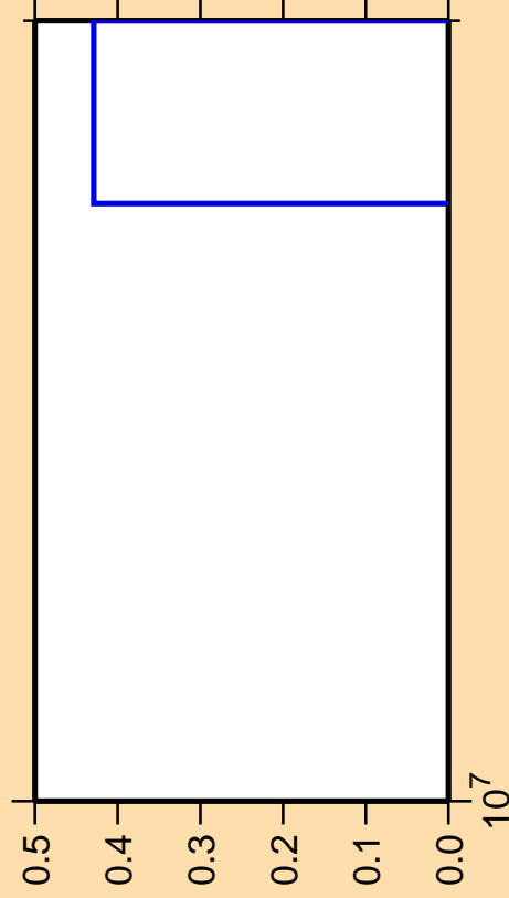
\Delta\sigma/\sigma vs. E for ^{124}\text{Cd}(n,nt)
