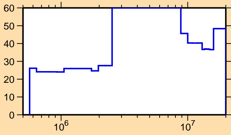
\Delta\sigma/\sigma vs. E for ^{124}\text{Cd}(n,\text{el.})
