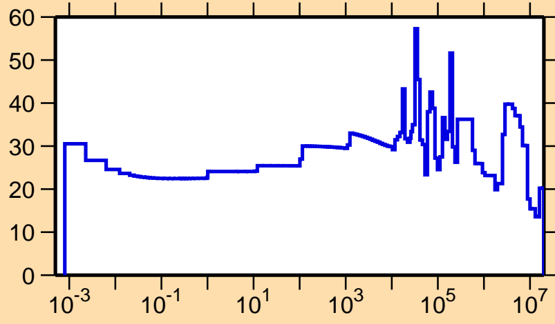
\Delta\sigma/\sigma vs. E for ^{124}\text{Cd}(n,\text{tot.})
