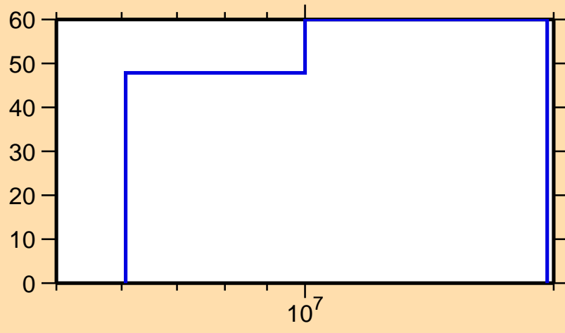
\Delta\sigma/\sigma vs. E for ^{124}\text{Cd}(n,\text{inel.})
