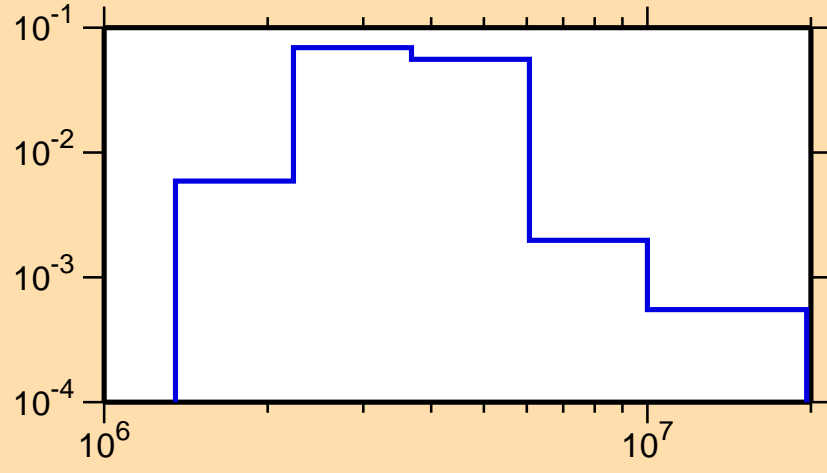
\sigma vs. E for ^{124}\text{Cd}(n,n_4)
