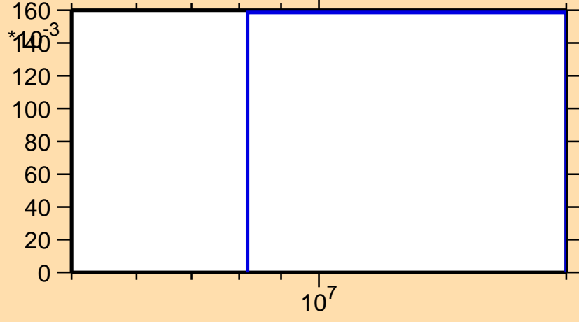
\sigma vs. E for ^{124}\text{Cd}(n,3n)
