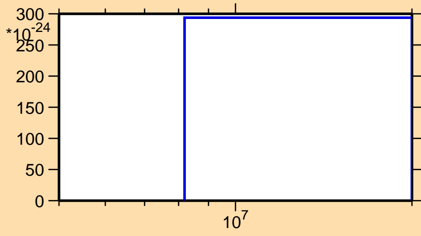
\sigma vs. E for ^{124}\text{Cd}(n,\text{nd})
