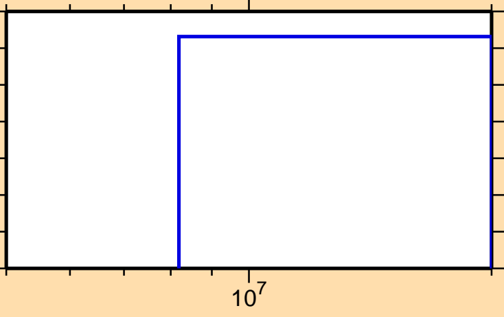
\sigma vs. E for ^{124}\text{Cd}(n,\alpha)
