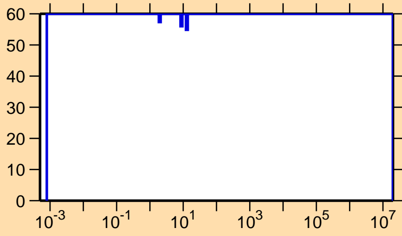
\Delta\sigma/\sigma vs. E for ^{121}\text{Ce}(n,\gamma)
