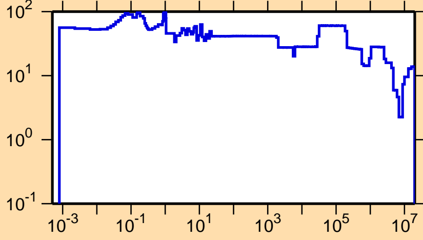
\Delta\sigma/\sigma vs. E for ^{121}\text{Ce}(n,\text{tot.})
