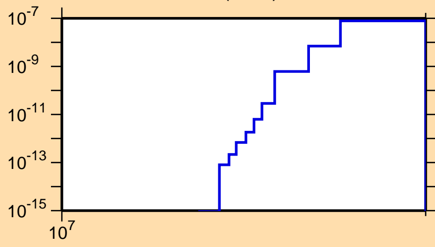
\sigma vs. E for ^{121}\text{Ce}(n,\text{nd})
