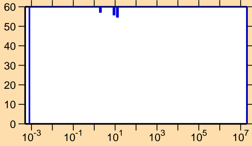
\Delta\sigma/\sigma vs. E for ^{121}\text{Ce}(n,\gamma)
