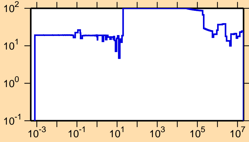
\Delta\sigma/\sigma vs. E for ^{121}\text{Ce}(n,\text{el.})
