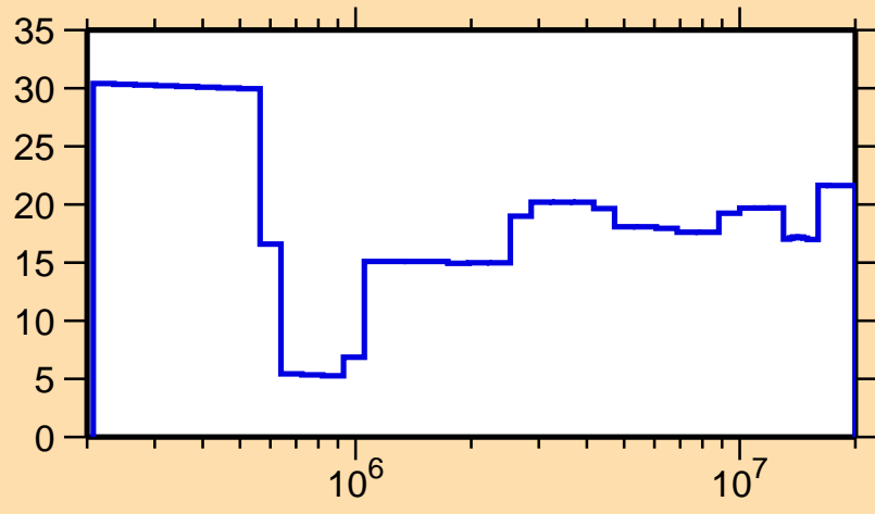
\Delta\sigma/\sigma vs. E for ^{121}\text{Ce}(n,\text{nonel.})
