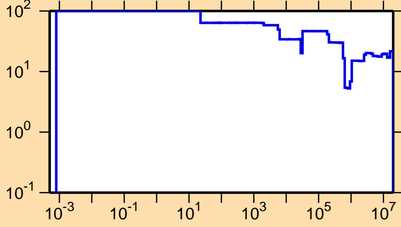
\Delta\sigma/\sigma vs. E for ^{121}\text{Ce}(n,\text{nonel.})
