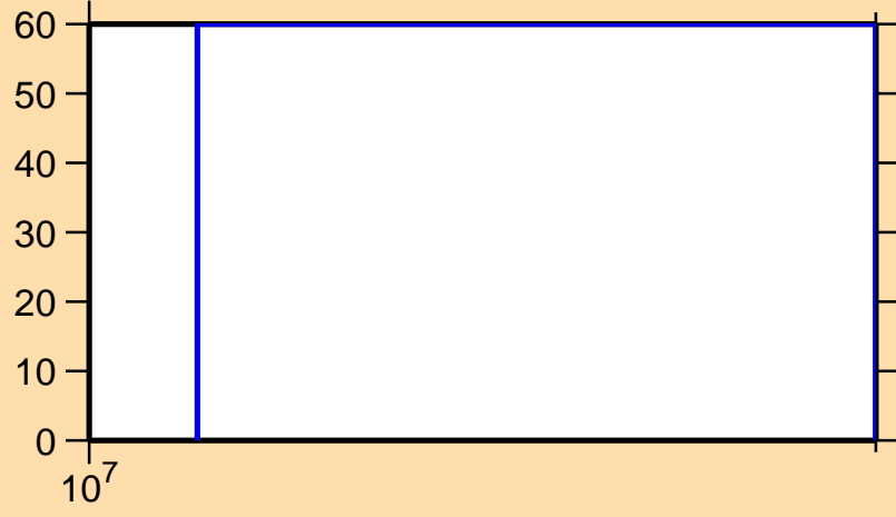
\Delta\sigma/\sigma vs. E for ^{121}\text{Ce}(n,\text{inel.})
