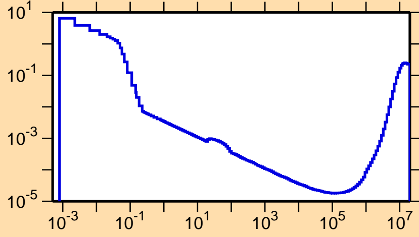
\sigma vs. E for ^{121}\text{Ce}(n,p\alpha)
