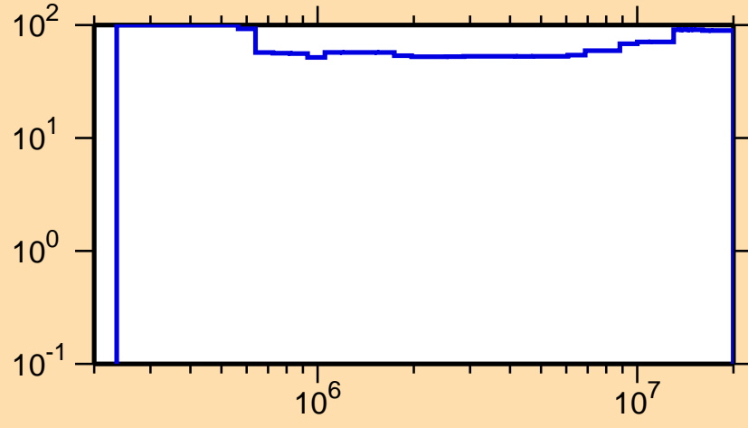
\Delta\sigma/\sigma vs. E for ^{121}\text{Ce}(n,n_1)
