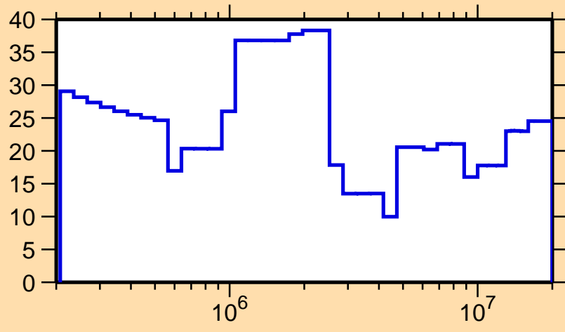
\Delta\sigma/\sigma vs. E for ^{121}\text{Ce}(n,\text{el.})
