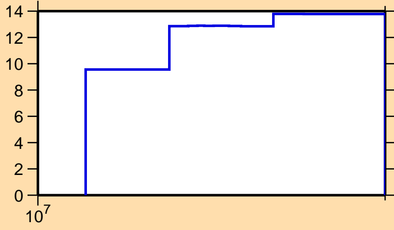
\Delta\sigma/\sigma vs. E for ^{121}\text{Ce}(n,\text{tot.})
