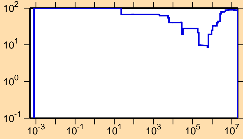
\Delta\sigma/\sigma vs. E for ^{121}\text{Ce}(n,p)
