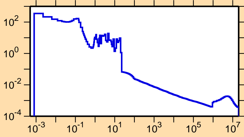
\sigma vs. E for ^{121}\text{Ce}(n,\gamma)
