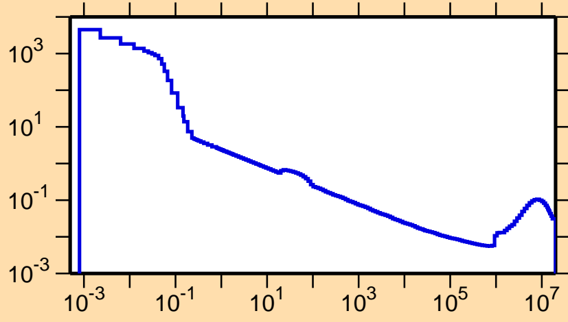
\sigma vs. E for ^{121}\text{Ce}(n,\alpha)
