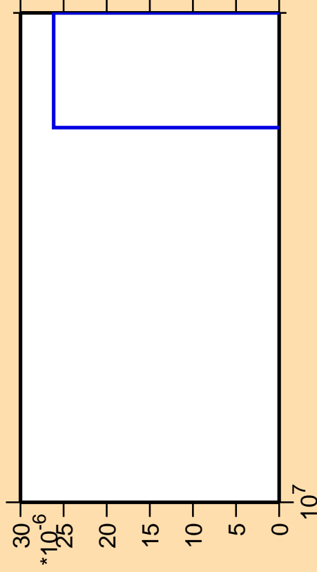
\Delta\sigma/\sigma vs. E for ^{121}\text{Ce}(n,nt)
