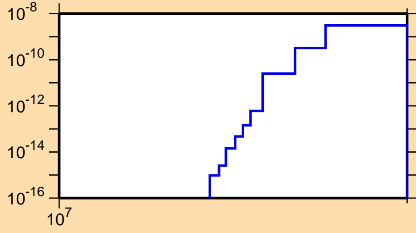
\sigma vs. E for ^{121}\text{Ce}(n,2n\alpha)
