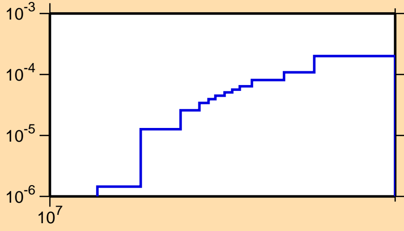
\sigma vs. E for ^{121}\text{Ce}(n,2n)
