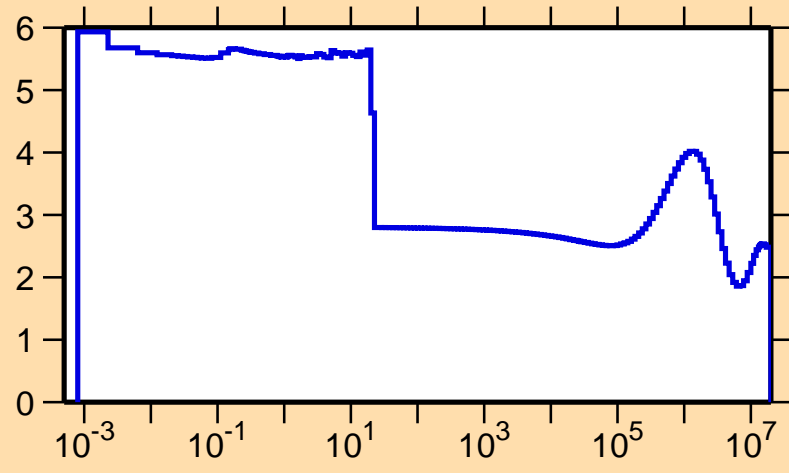
\sigma vs. E for ^{121}\text{Ce}(n,\text{el.})
