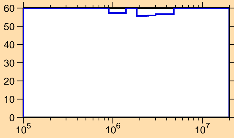
\Delta\sigma/\sigma vs. E for ^{121}\text{Ce}(n,\text{inel.})
