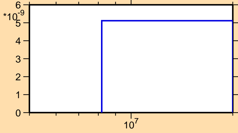
\sigma vs. E for ^{121}\text{Ce}(\text{mt } 34)
