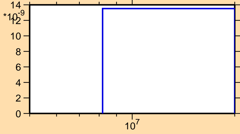
\sigma vs. E for ^{121}\text{Ce}(\text{mt117})
