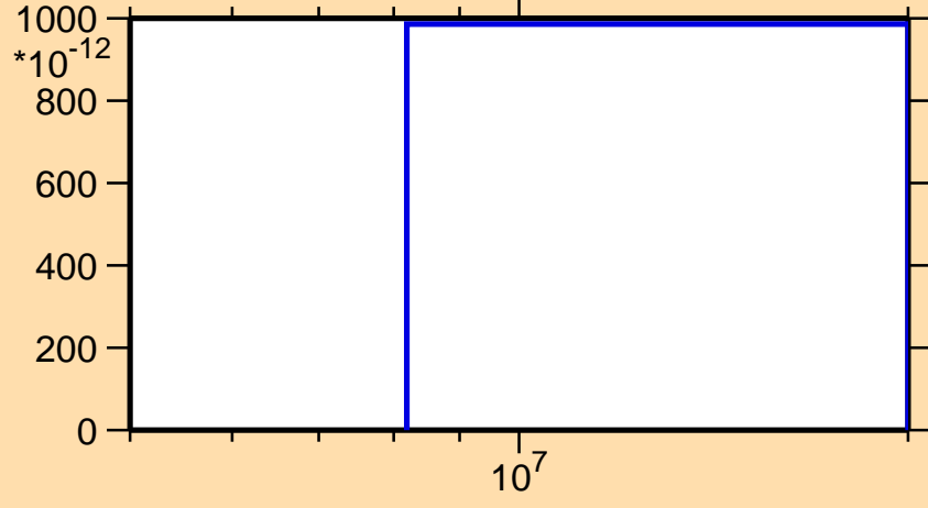
\sigma vs. E for ^{121}\text{Ce}(n,\text{nd})
