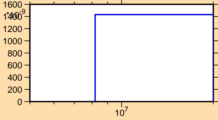
\sigma vs. E for ^{121}\text{Ce}(\text{mt } 45)
