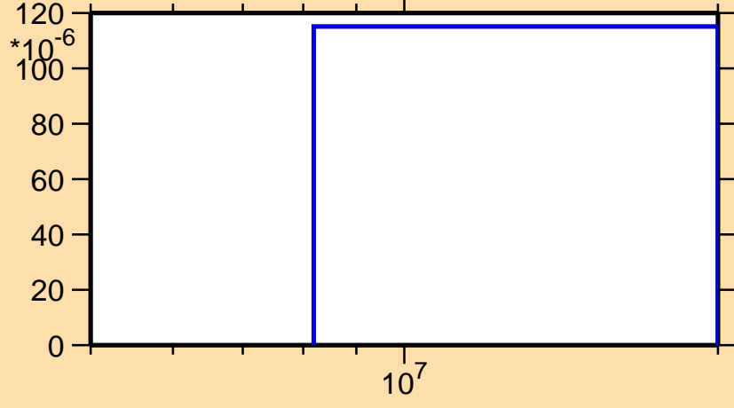
\sigma vs. E for ^{121}\text{Ce}(n,\text{pt})
