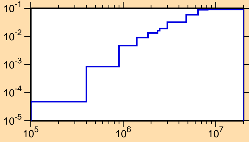
\sigma vs. E for ^{121}\text{Ce}(n,n\text{cont.})
