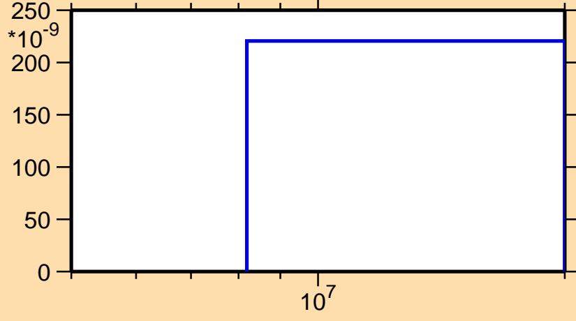
\sigma vs. E for ^{121}\text{Ce}(n,2np)
