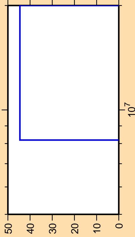
\Delta\sigma/\sigma vs. E for ^{121}\text{Ce}(\text{mt } 45)
