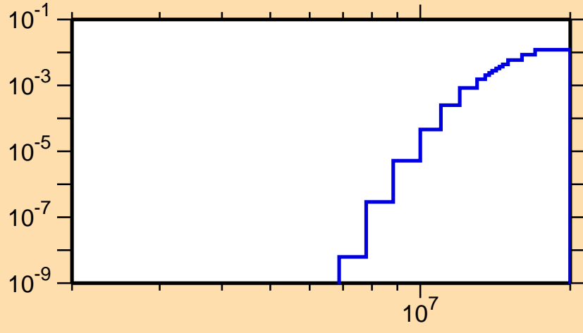
\sigma vs. E for ^{122}\text{Ce}(n,pd)
