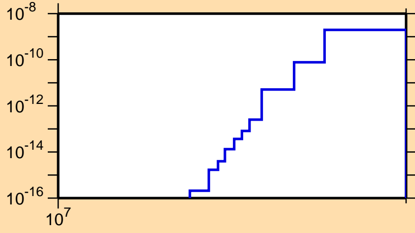
\sigma vs. E for ^{122}\text{Ce}(\text{mt } 34)
