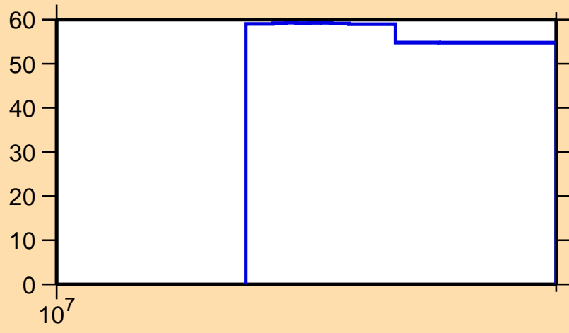
\Delta\sigma/\sigma vs. E for ^{122}\text{Ce}(n,\text{inel.})
