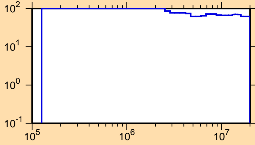
\Delta\sigma/\sigma vs. E for ^{122}\text{Ce}(n,n_1)
