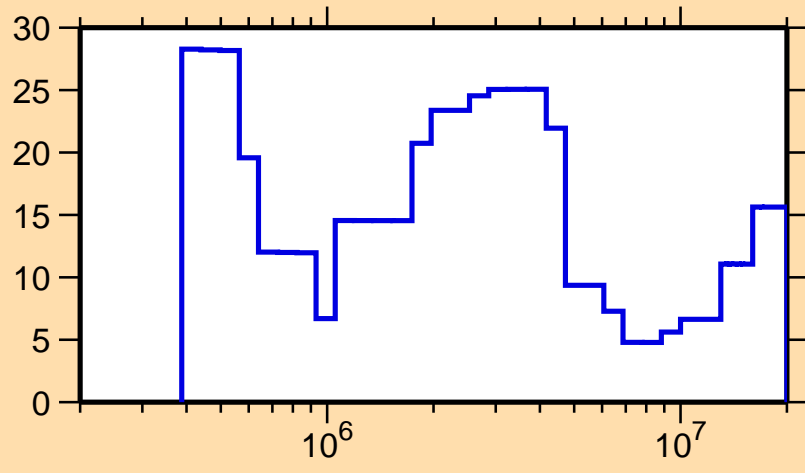
\Delta\sigma/\sigma vs. E for ^{122}\text{Ce}(n,\text{el.})
