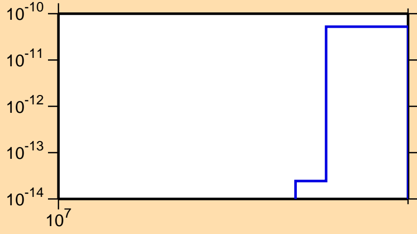
\sigma vs. E for ^{122}\text{Ce}(n,2n\alpha)
