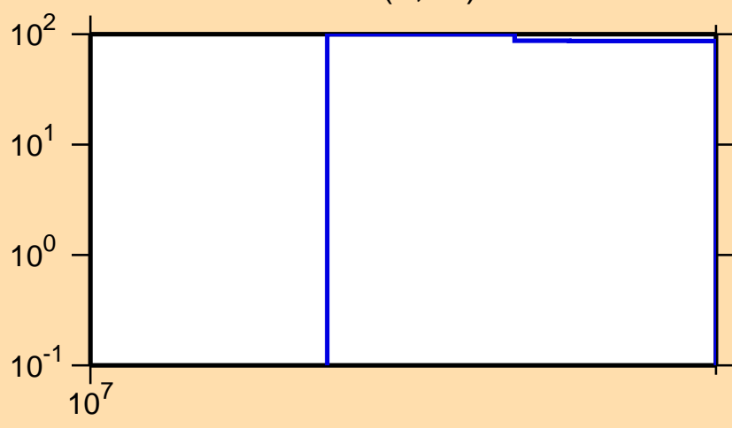
\Delta\sigma/\sigma vs. E for ^{122}\text{Ce}(n,2n)
