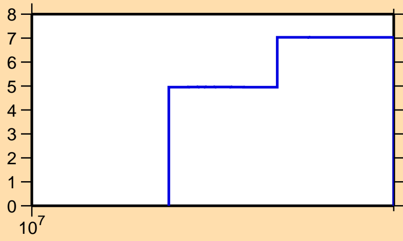
\Delta\sigma/\sigma vs. E for ^{122}\text{Ce}(n,\text{tot.})
