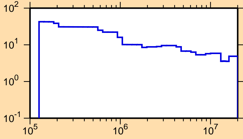
\Delta\sigma/\sigma vs. E for ^{122}\text{Ce}(n,\text{nonel.})
