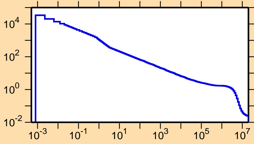
\sigma vs. E for ^{122}\text{Ce}(n,p)
