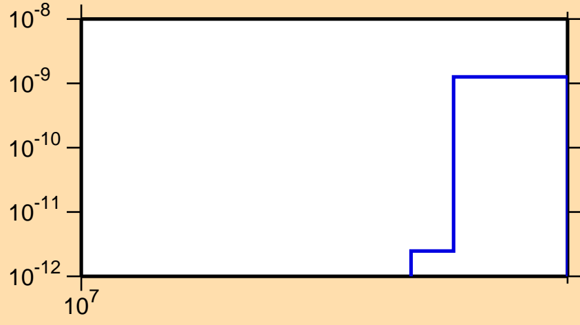
\sigma vs. E for ^{122}\text{Ce}(n,\text{nd})
