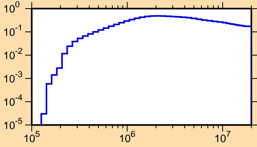
\sigma vs. E for ^{122}\text{Ce}(n,\text{inel.})
