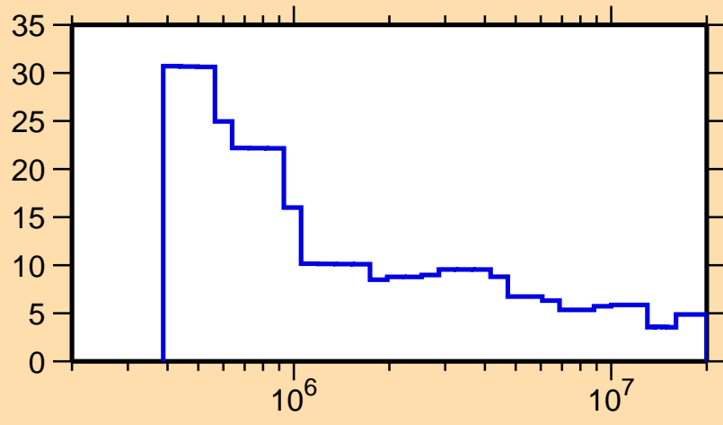
\Delta\sigma/\sigma vs. E for ^{122}\text{Ce}(n,\text{nonel.})
