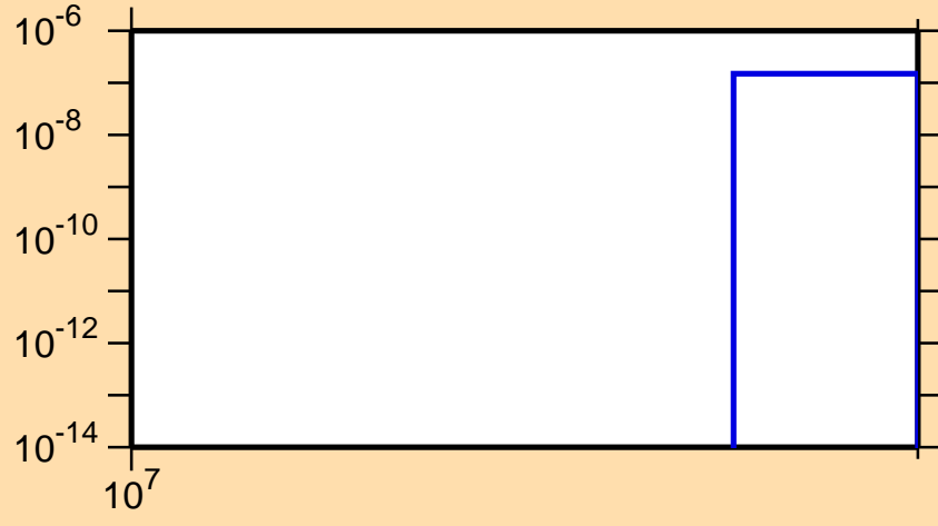
\sigma vs. E for ^{122}\text{Ce}(n,2np)
