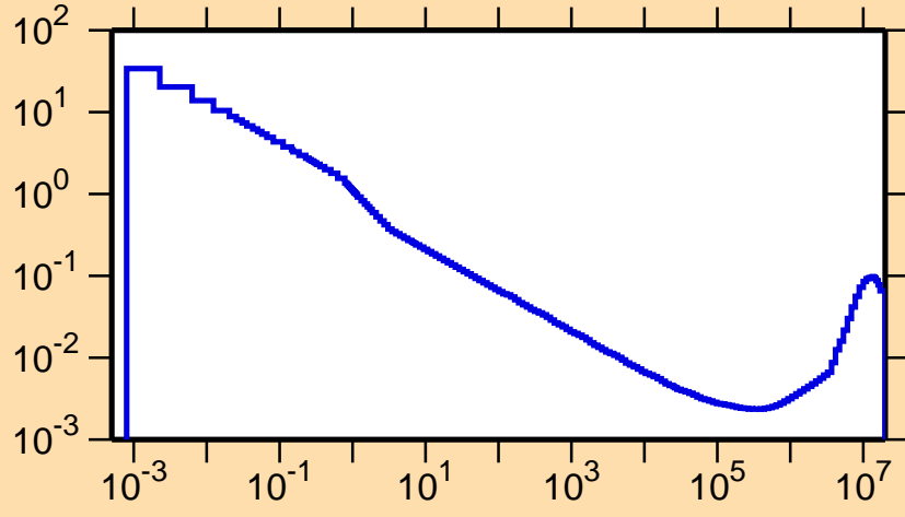
\sigma vs. E for ^{122}\text{Ce}(n,\alpha)
