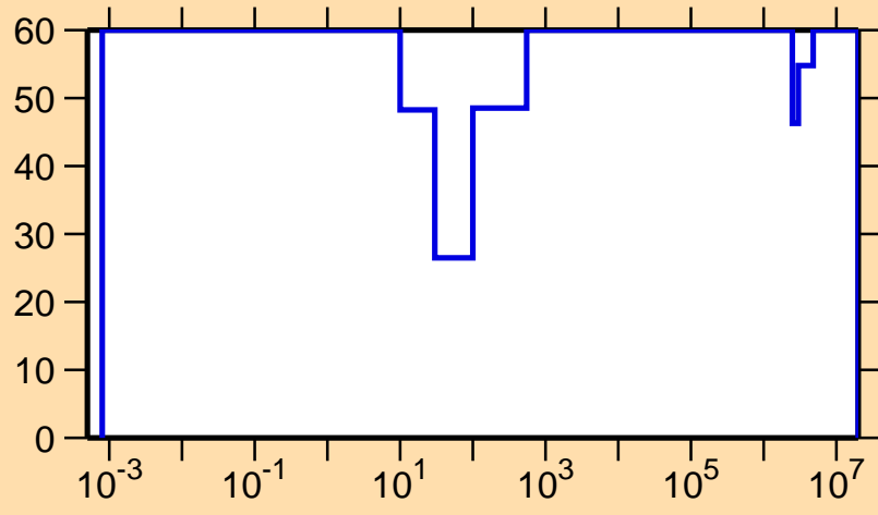
\Delta\sigma/\sigma vs. E for ^{122}\text{Ce}(n,\gamma)
