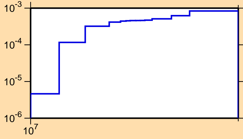
\sigma vs. E for ^{123}\text{Ce}(n,2n)
