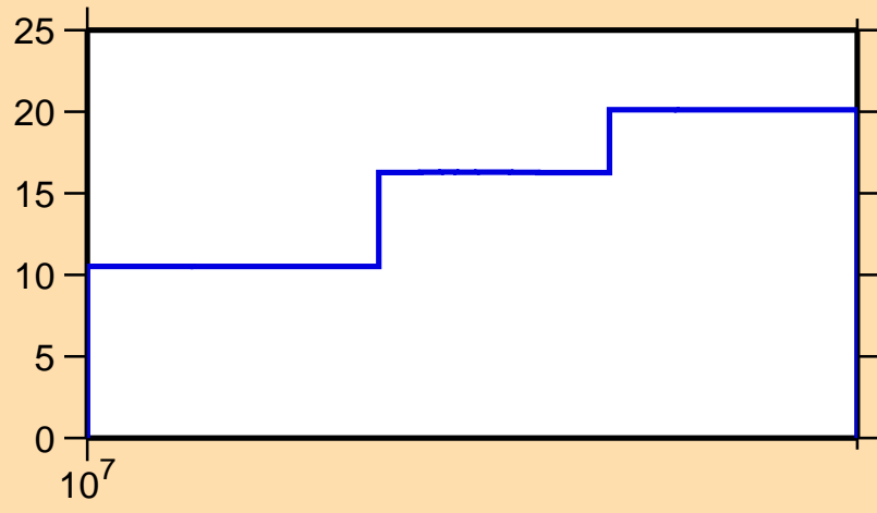
\Delta\sigma/\sigma vs. E for ^{123}\text{Ce}(n,\text{tot.})
