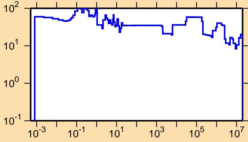
\Delta\sigma/\sigma vs. E for ^{123}\text{Ce}(n,\text{tot.})
