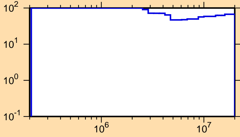
\Delta\sigma/\sigma vs. E for ^{123}\text{Ce}(n,\text{inel.})
