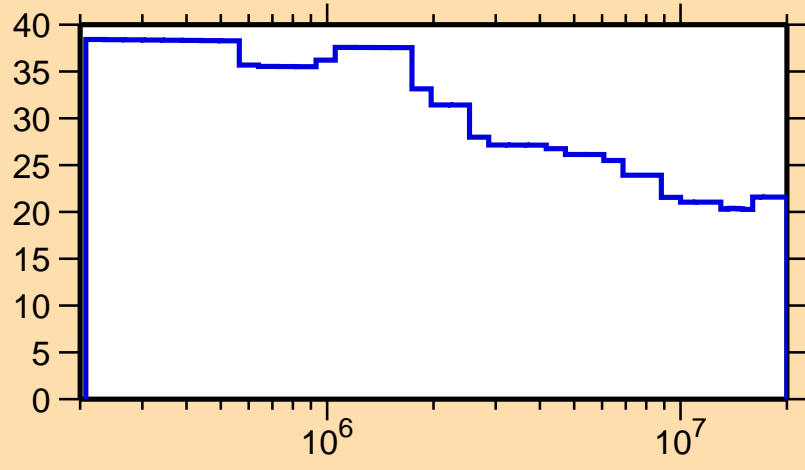
\Delta\sigma/\sigma vs. E for ^{123}\text{Ce}(n,\text{nonel.})
