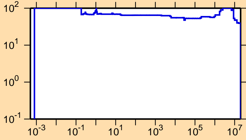
\Delta\sigma/\sigma vs. E for ^{123}\text{Ce}(n,p)
