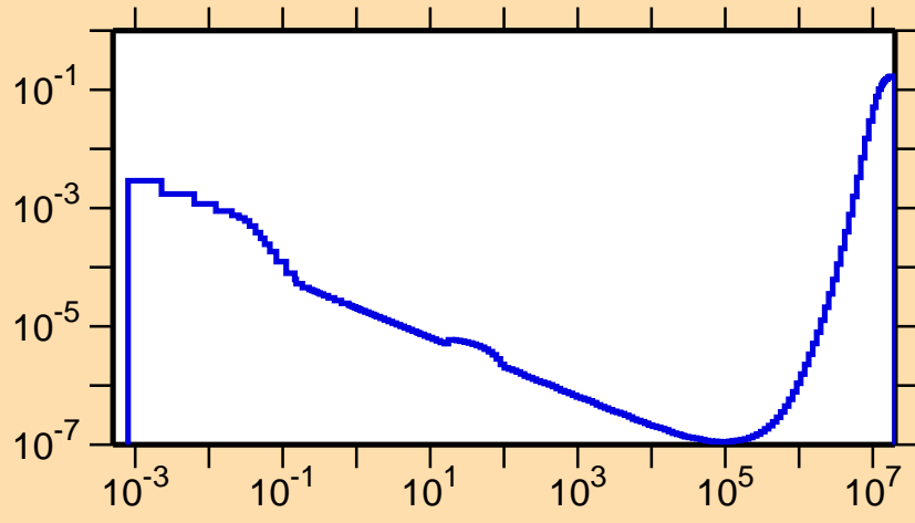
\sigma vs. E for ^{123}\text{Ce}(n,p\alpha)
