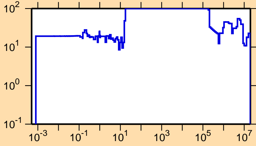
\Delta\sigma/\sigma vs. E for ^{123}\text{Ce}(n,\text{el.})
