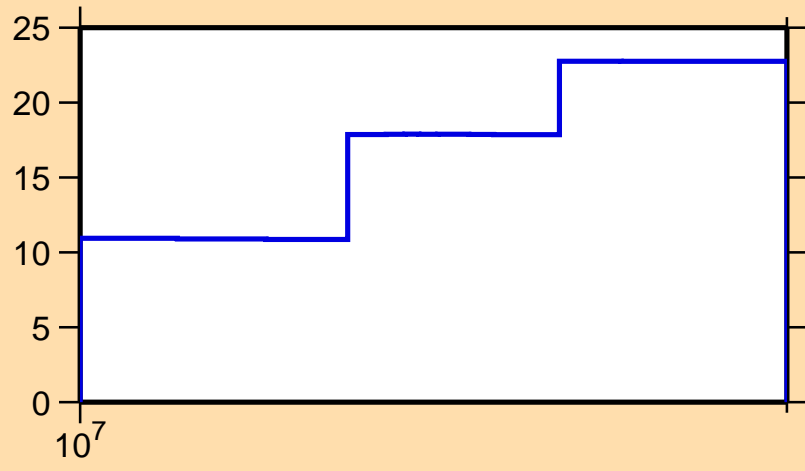
\Delta\sigma/\sigma vs. E for ^{123}\text{Ce}(n,\text{el.})
