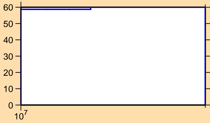
\Delta\sigma/\sigma vs. E for ^{123}\text{Ce}(n,\text{inel.})
