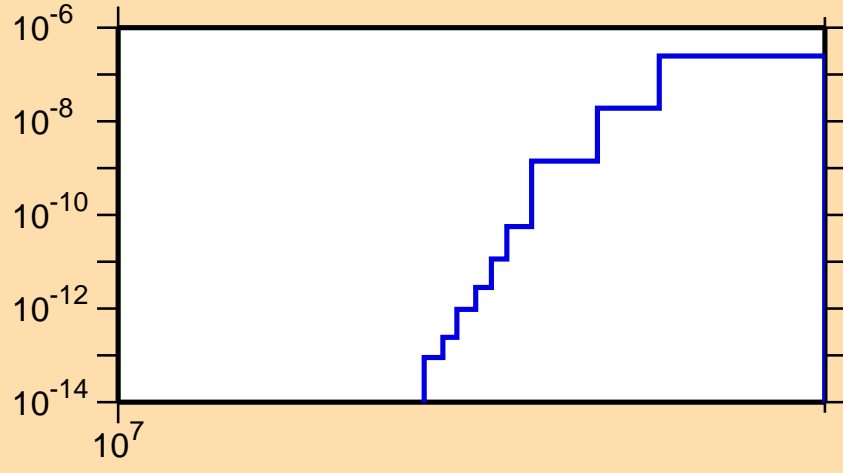
\sigma vs. E for ^{123}\text{Ce}(n,\text{nd})
