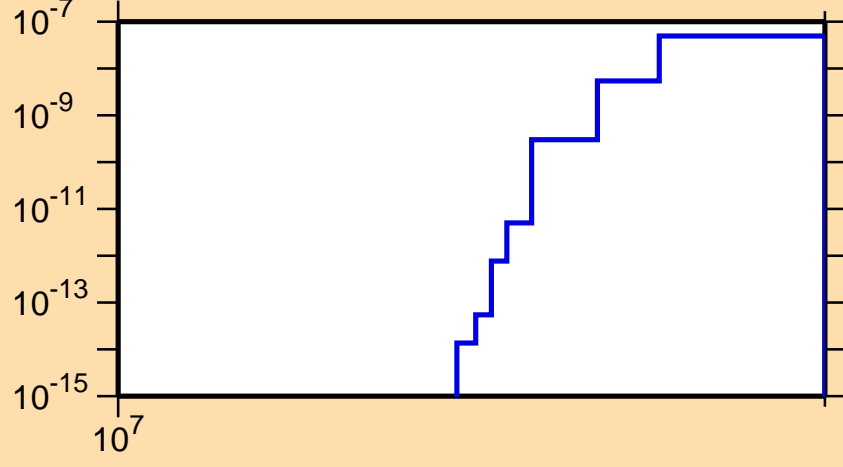
\sigma vs. E for ^{123}\text{Ce}(n,2n\alpha)
