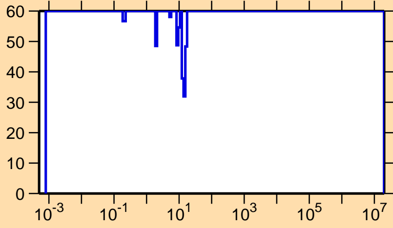
\Delta\sigma/\sigma vs. E for ^{123}\text{Ce}(n,\gamma)
