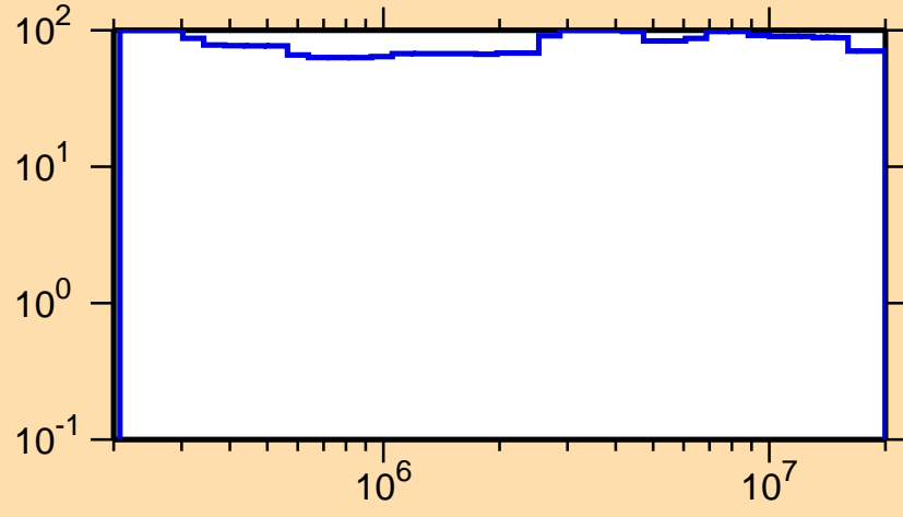
\Delta\sigma/\sigma vs. E for ^{123}\text{Ce}(n,n_1)
