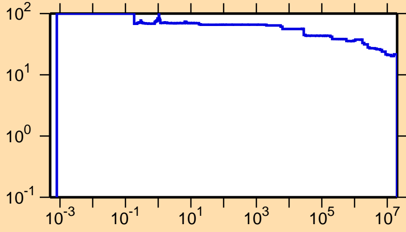
\Delta\sigma/\sigma vs. E for ^{123}\text{Ce}(n,\text{nonel.})
