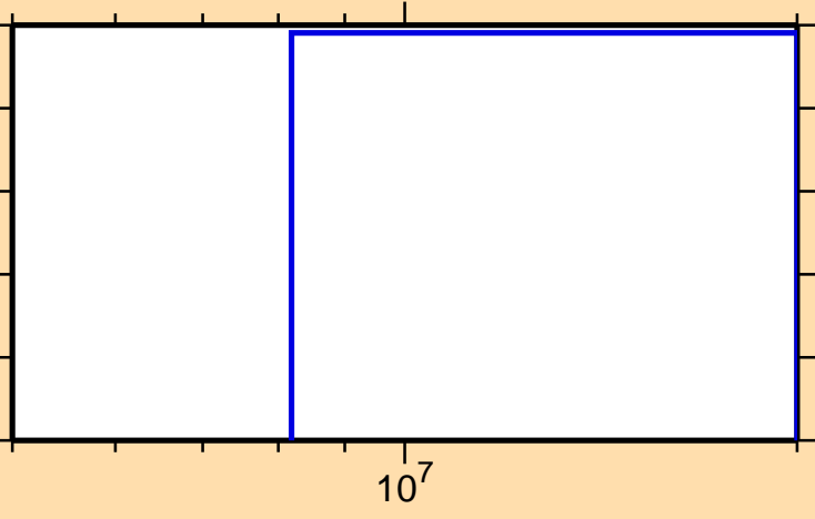
\sigma vs. E for ^{123}\text{Ce} (mt 45)
