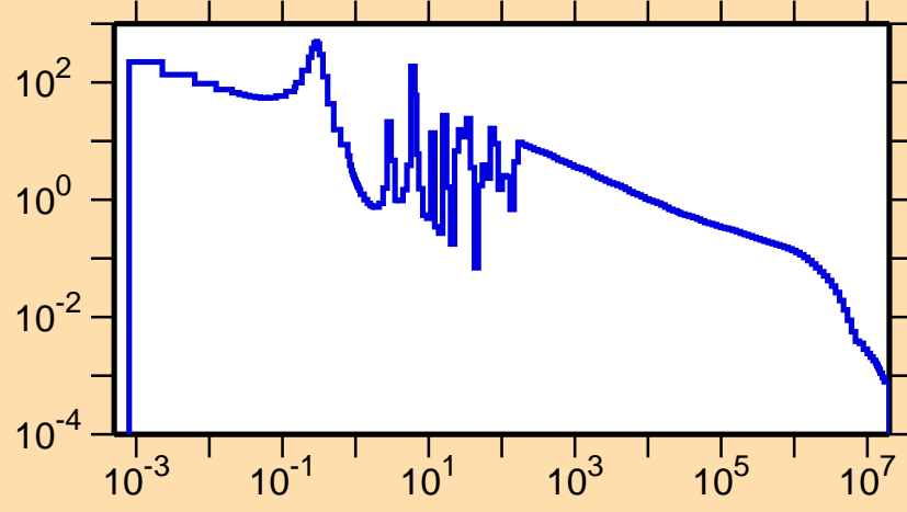
\sigma vs. E for ^{124}\text{Ce}(n,\gamma)
