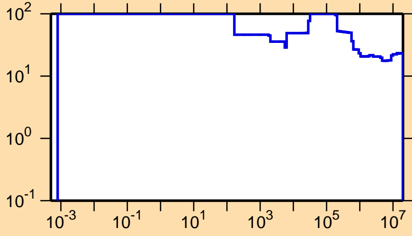
\Delta\sigma/\sigma vs. E for ^{124}\text{Ce}(n,\text{nonel.})
