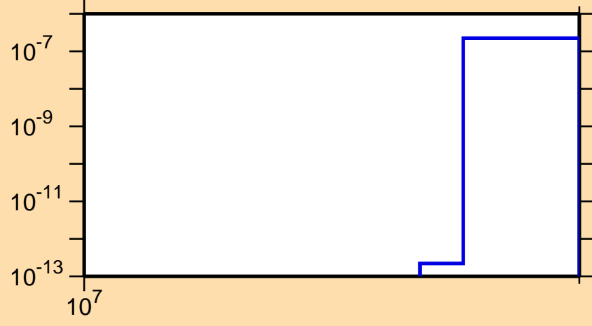
\sigma vs. E for ^{124}\text{Ce}(n,2np)
