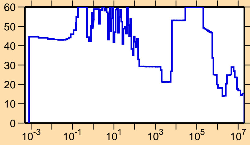
\Delta\sigma/\sigma vs. E for ^{124}\text{Ce}(n,\text{tot.})
