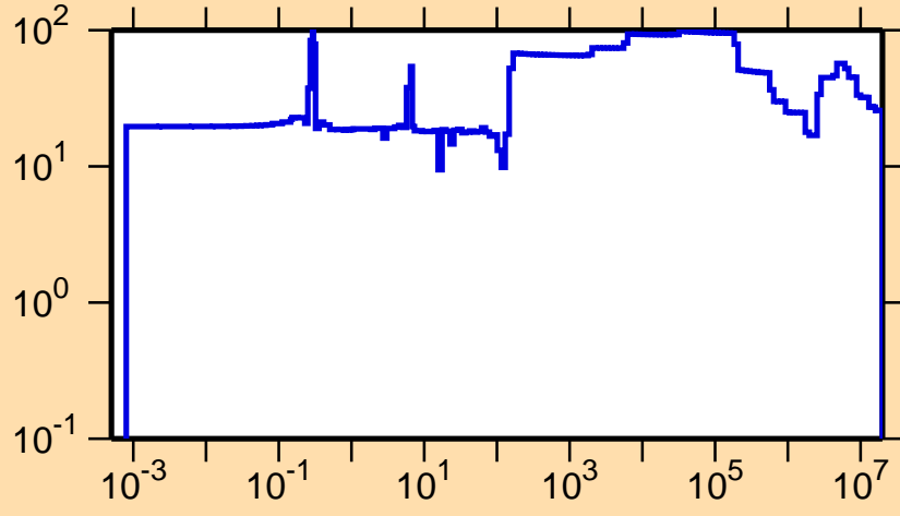
\Delta\sigma/\sigma vs. E for ^{124}\text{Ce}(n,\text{el.})
