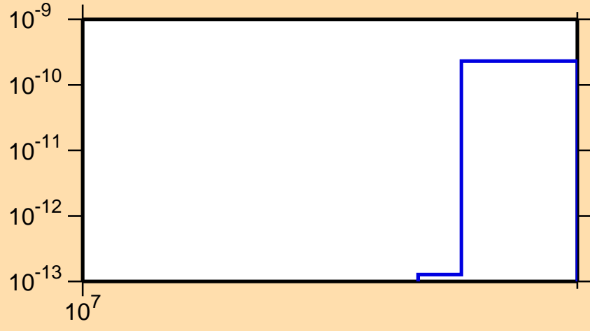
\sigma vs. E for ^{124}\text{Ce}(n,2n\alpha)
