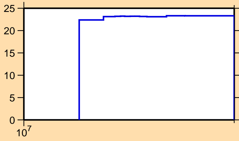
\Delta\sigma/\sigma vs. E for ^{124}\text{Ce}(n,\text{nonel.})
