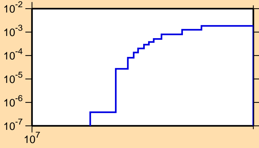
\sigma vs. E for ^{124}\text{Ce}(n,2n)
