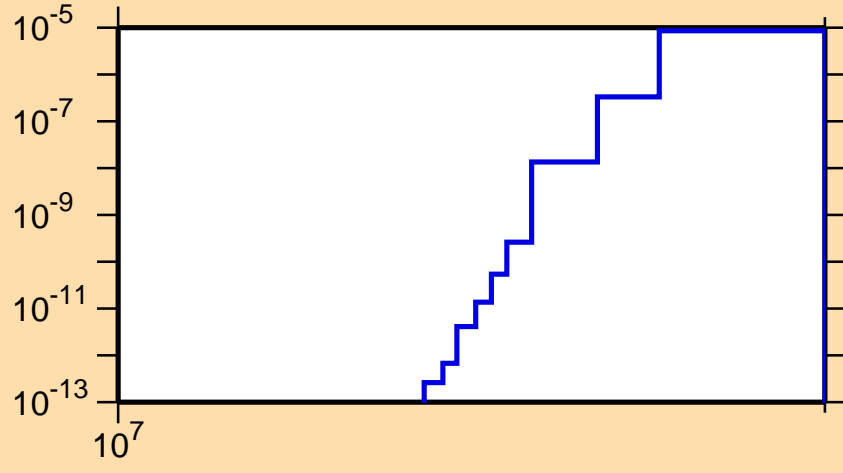
\sigma vs. E for ^{124}\text{Ce}(n,\text{pt})
