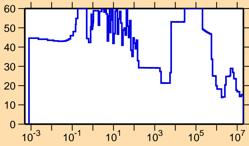
\Delta\sigma/\sigma vs. E for ^{124}\text{Ce}(n,\text{tot.})
