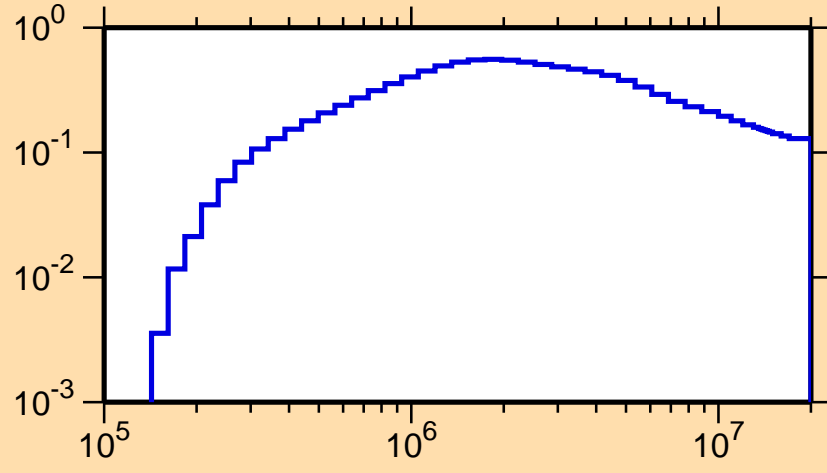
\sigma vs. E for ^{124}\text{Ce}(n,\text{inel.})
