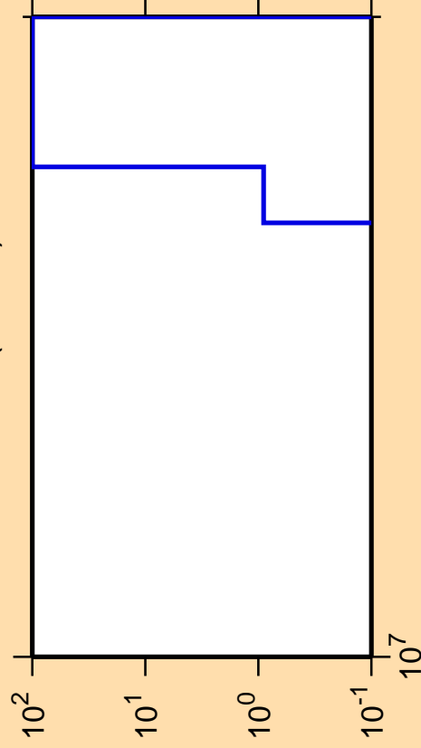
\Delta\sigma/\sigma vs. E for ^{124}\text{Ce}(n,2n\alpha)
