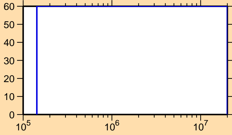
\Delta\sigma/\sigma vs. E for ^{124}\text{Ce}(n,n_1)
