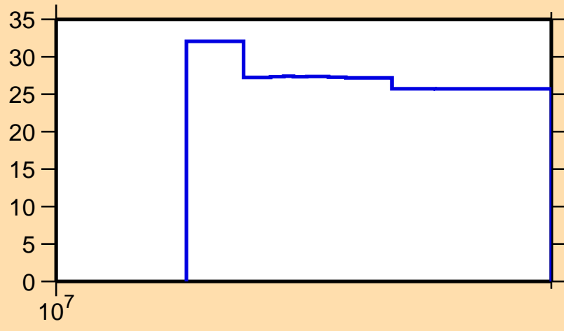
\Delta\sigma/\sigma vs. E for ^{124}\text{Ce}(n,\text{el.})
