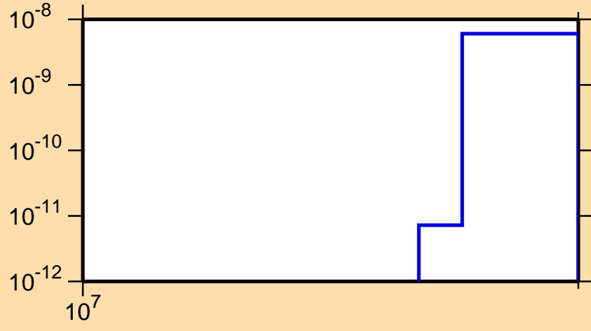
\sigma vs. E for ^{124}\text{Ce}(n,\text{nd})
