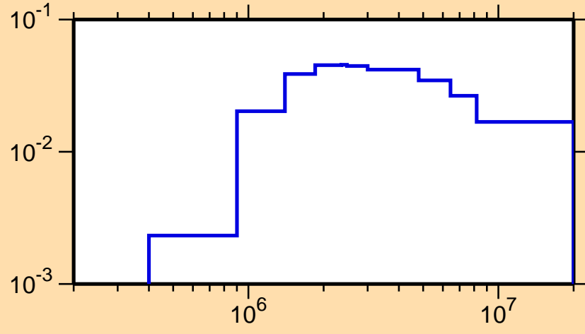
\sigma vs. E for ^{124}\text{Ce}(n,n_2)
