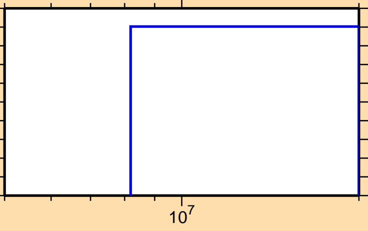
\sigma vs. E for ^{124}\text{Ce} (mt 34)
