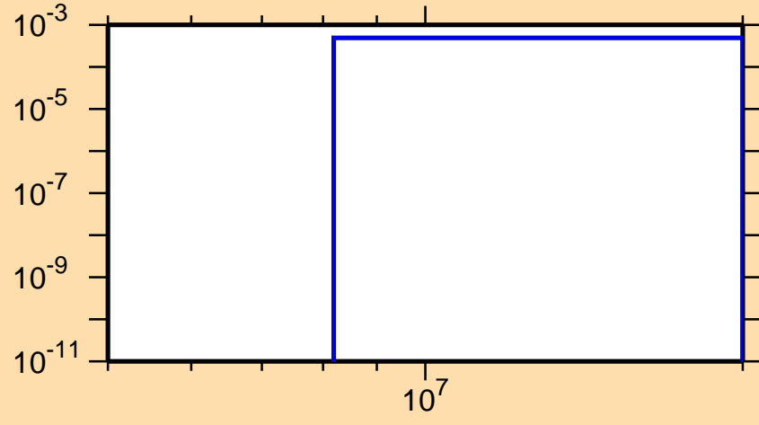
\sigma vs. E for ^{124}\text{Ce}(n,\text{pd})
