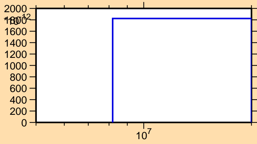
\sigma vs. E for ^{124}\text{Ce}(n,2np)
