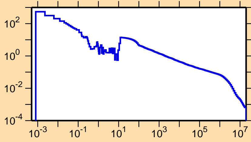
\sigma vs. E for ^{125}\text{Ce}(n,\gamma)
