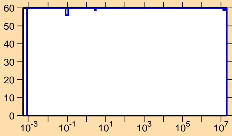
\Delta\sigma/\sigma vs. E for ^{125}\text{Ce}(n,\gamma)
