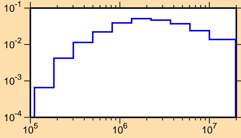
\sigma vs. E for ^{125}\text{Ce}(n,n_2)
