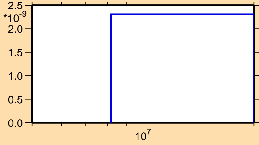
\sigma vs. E for ^{125}\text{Ce}(\text{mt } 34)
