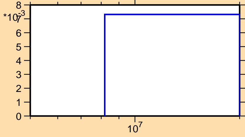
\sigma vs. E for ^{126}\text{Ce}(n,2n)
