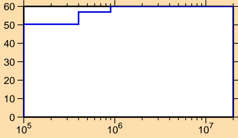
\Delta\sigma/\sigma vs. E for ^{126}\text{Ce}(n,n_1)
