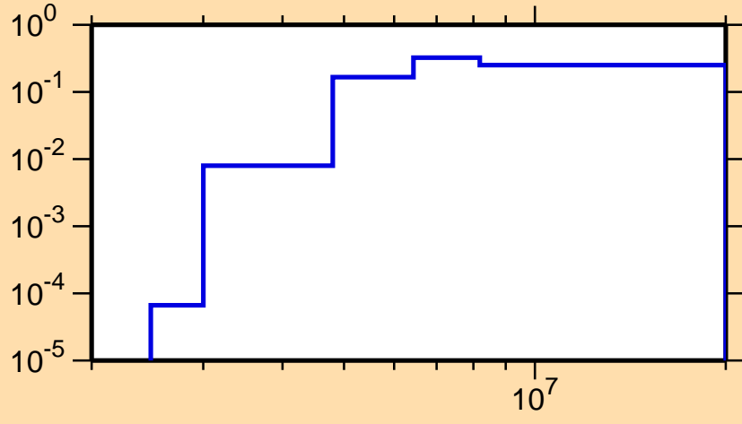
\sigma vs. E for ^{126}\text{Ce}(n,n\text{cont.})
