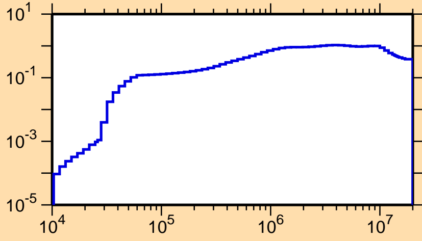
\sigma vs. E for ^{127}\text{Ce}(n,\text{inel.})
