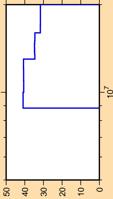
\Delta\sigma/\sigma vs. E for ^{127}\text{Ce}(n,n\text{cont.})
