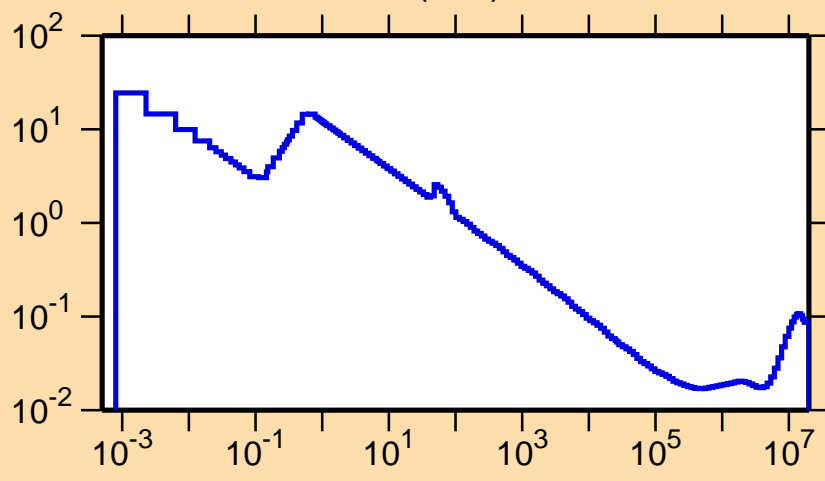
\sigma vs. E for ^{127}\text{Ce}(n,\alpha)
