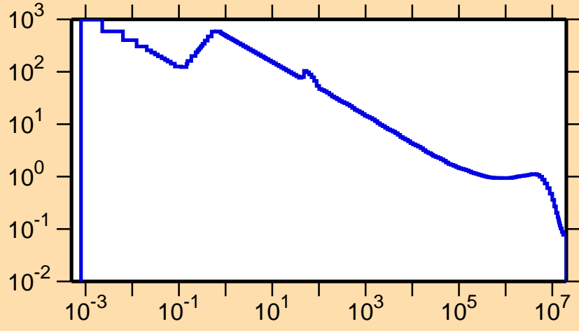
\sigma vs. E for ^{127}\text{Ce}(n,p)
