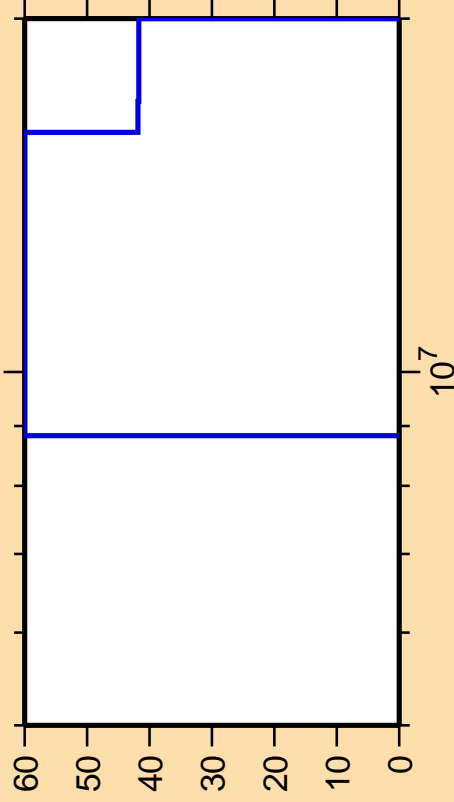
\Delta\sigma/\sigma vs. E for ^{127}\text{Ce}(n,p)
