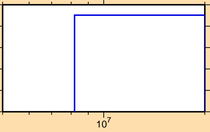
\sigma vs. E for ^{127}\text{Ce}(n,2n\alpha)
