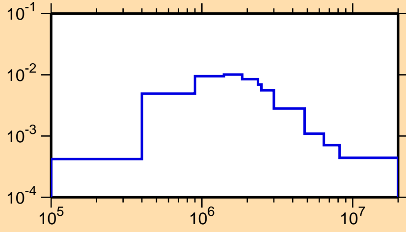
\sigma vs. E for ^{127}\text{Ce}(n,n_4)
