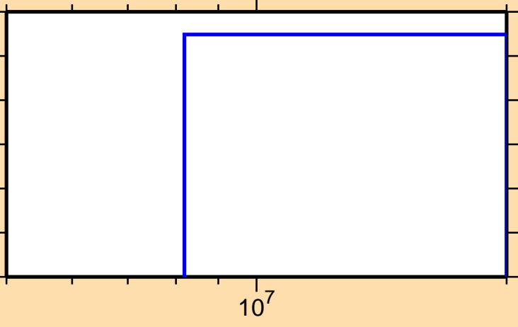
\sigma vs. E for ^{127}\text{Ce}(\text{mt } 45)
