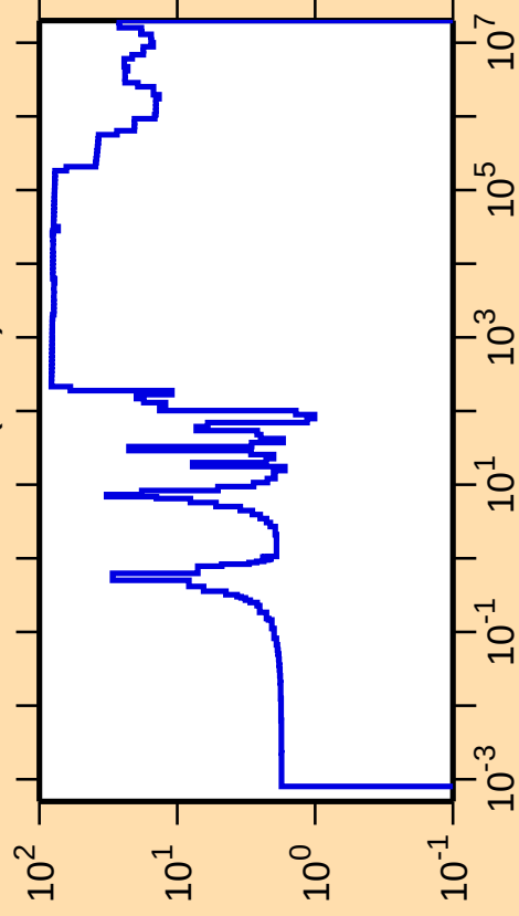
\Delta\sigma/\sigma vs. E for ^{128}\text{Ce}(n,\text{el.})
