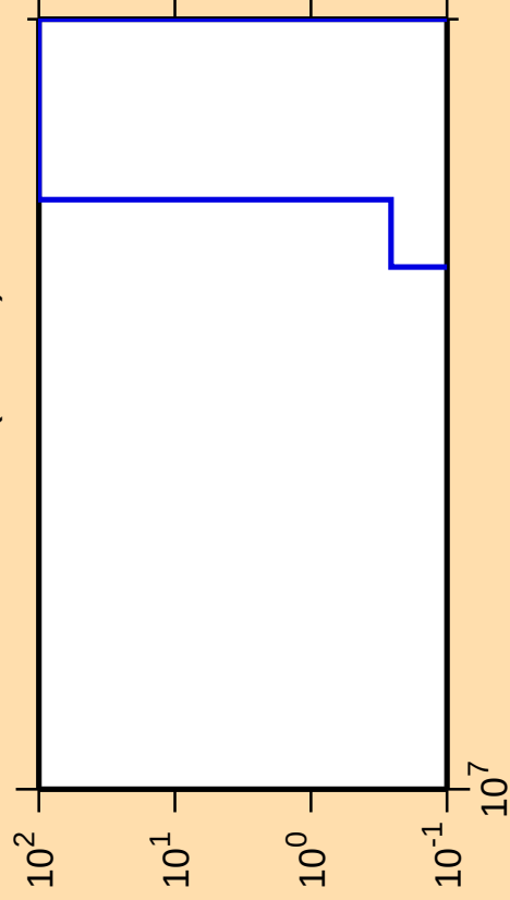
\Delta\sigma/\sigma vs. E for ^{128}\text{Ce}(\text{mt } 34)
