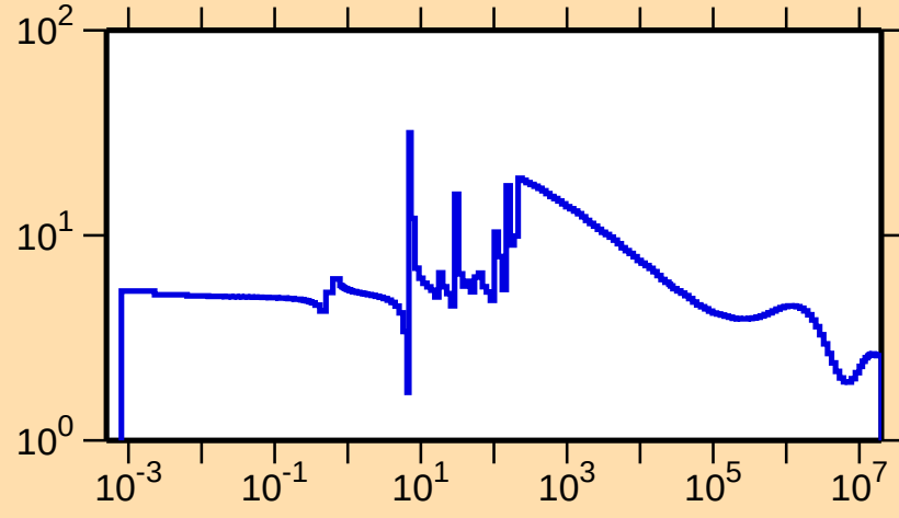
\sigma vs. E for ^{128}\text{Ce}(n,\text{el.})
