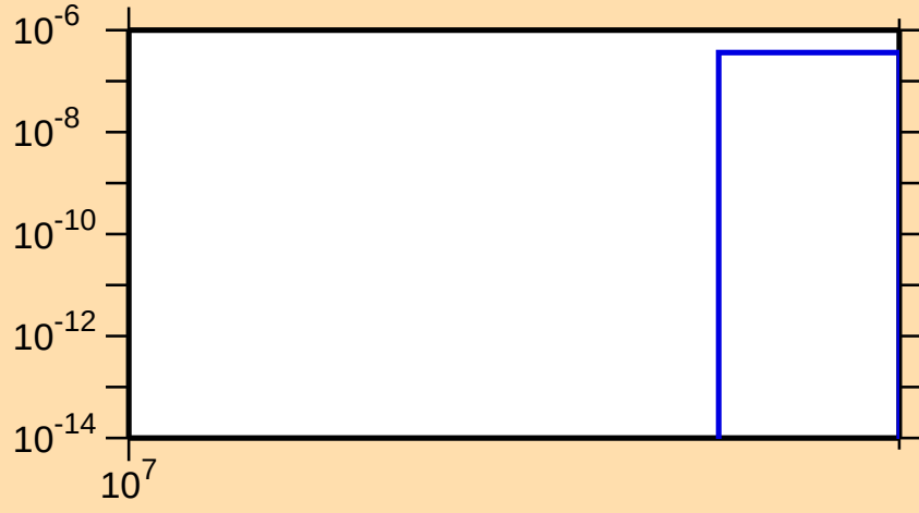
\sigma vs. E for ^{128}\text{Ce}(n,2np)
