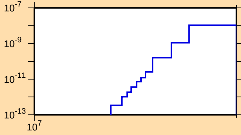
\sigma vs. E for ^{128}\text{Ce}(\text{mt117})
