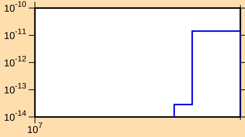
\sigma vs. E for ^{128}\text{Ce}(\text{mt } 34)
