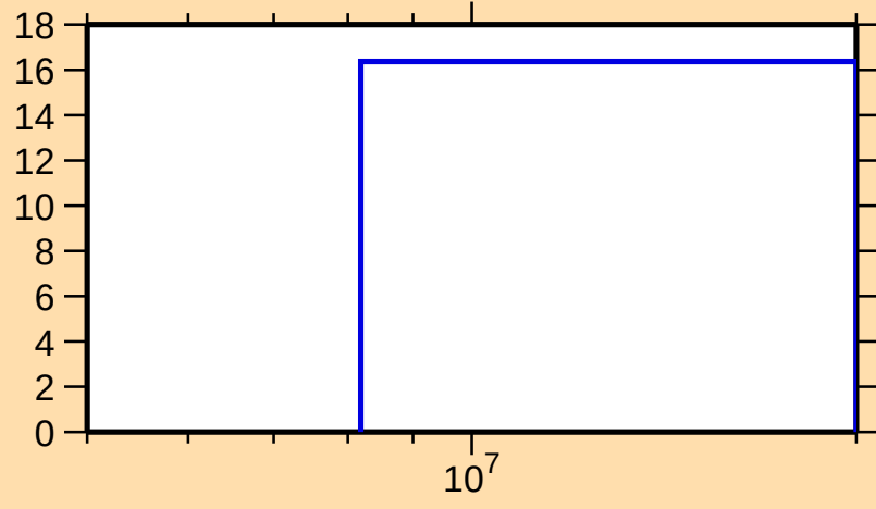
\Delta\sigma/\sigma vs. E for ^{128}\text{Ce}(n,\text{nonel.})
