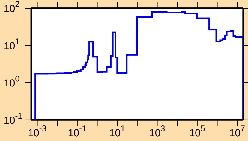
\Delta\sigma/\sigma vs. E for ^{128}\text{Ce}(n,\text{el.})
