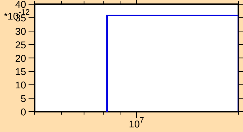
\sigma vs. E for ^{128}\text{Ce}(n,\text{pt})
