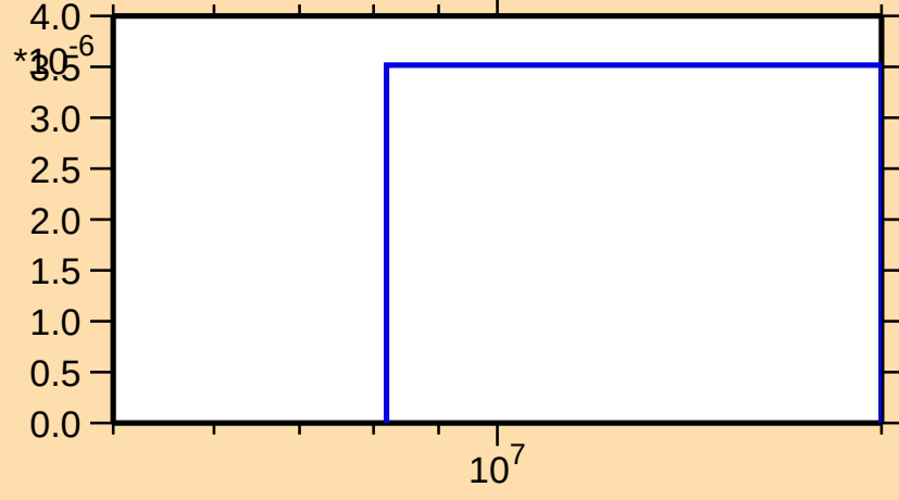
\sigma vs. E for ^{128}\text{Ce}(n,\text{pd})
