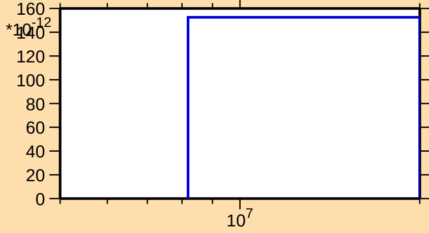
\sigma vs. E for ^{128}\text{Ce}(\text{mt117})
