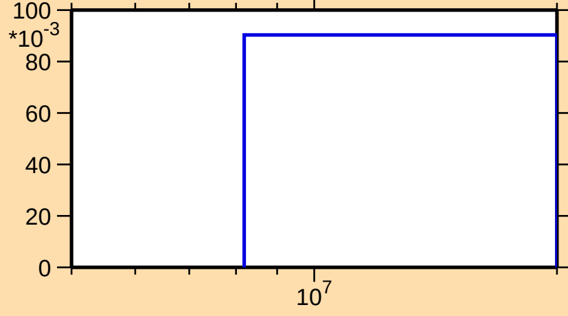
\sigma vs. E for ^{128}\text{Ce}(n,2n)
