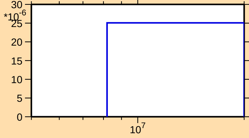
\sigma vs. E for ^{128}\text{Ce}(n,t)
