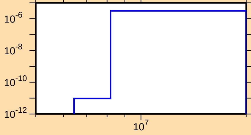
\sigma vs. E for ^{128}\text{Ce}(n,\text{He}3)
