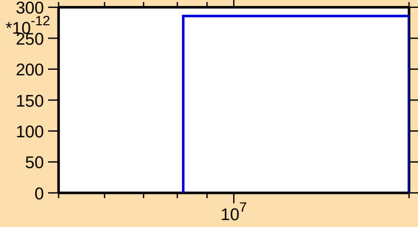
\sigma vs. E for ^{128}\text{Ce}(n,\text{nd})
