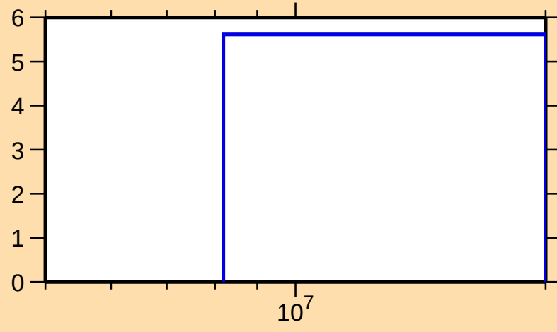
\Delta\sigma/\sigma vs. E for ^{128}\text{Ce}(n,\text{tot.})
