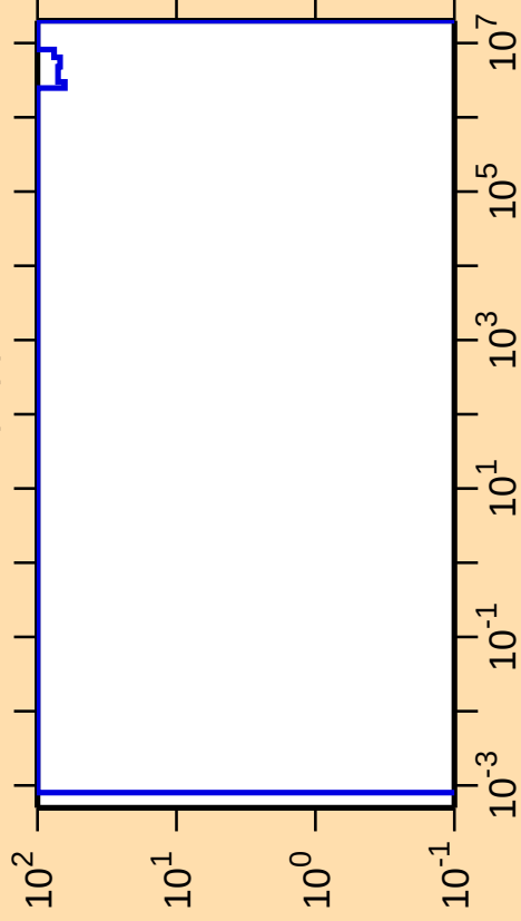
\Delta\sigma/\sigma vs. E for ^{128}\text{Ce}(n,p)
