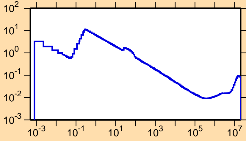
\sigma vs. E for ^{129}\text{Ce}(n,\alpha)
