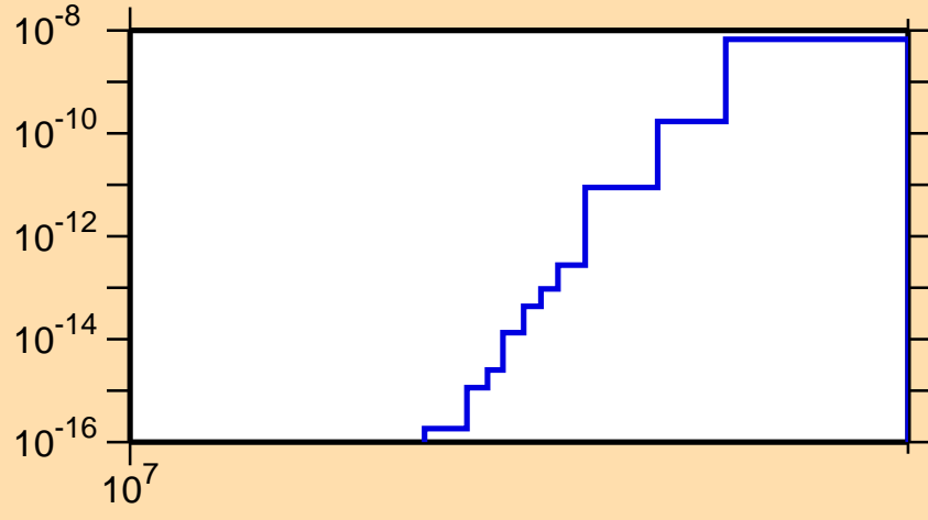
\sigma vs. E for ^{129}\text{Ce}(\text{mt } 34)
