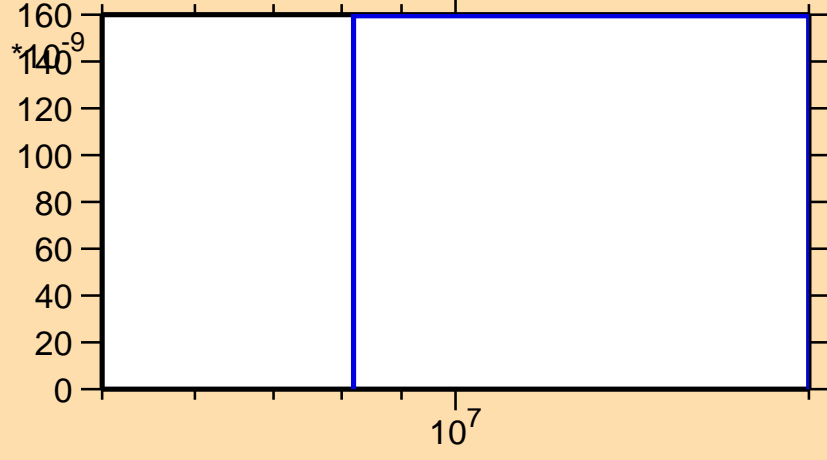
\sigma vs. E for ^{129}\text{Ce}(n,\text{nd})
