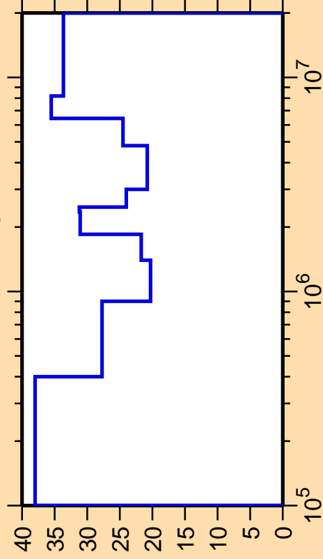
\Delta\sigma/\sigma vs. E for ^{129}\text{Ce}(n,n_3)
