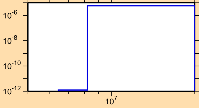
\sigma vs. E for ^{129}\text{Ce}(n,\text{He}3)
