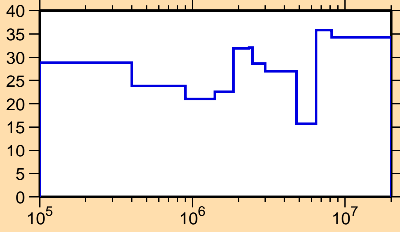
\Delta\sigma/\sigma vs. E for ^{129}\text{Ce}(n,n_1)
