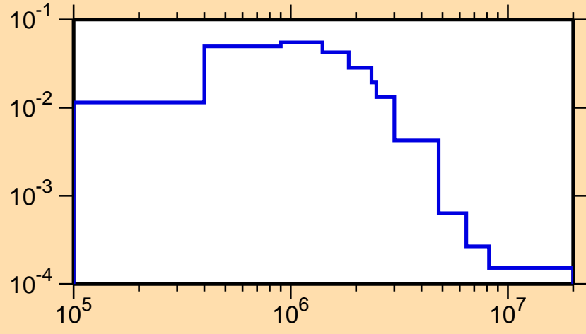
\sigma vs. E for ^{129}\text{Ce}(n,n_3)
