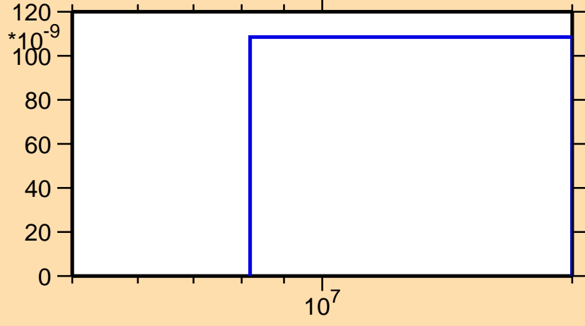
\sigma vs. E for ^{129}\text{Ce}(n,2n\alpha)
