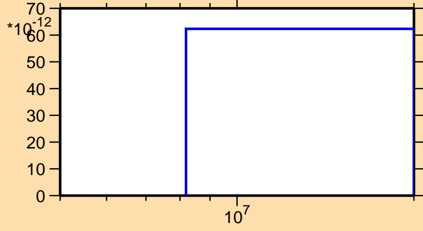
\sigma vs. E for ^{129}\text{Ce}(\text{mt } 34)
