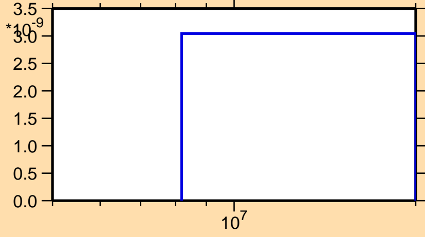
\sigma vs. E for ^{129}\text{Ce}(\text{mt } 45)
