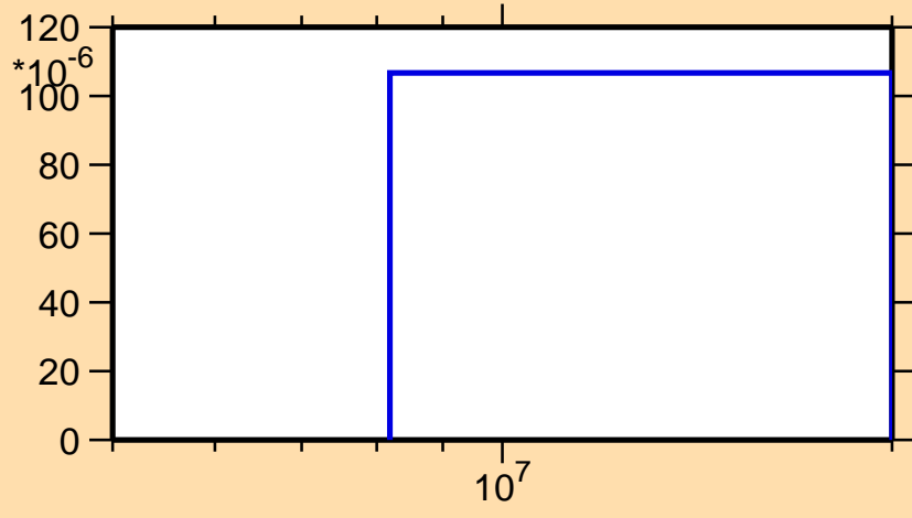
\sigma vs. E for ^{129}\text{Ce}(n,t)
