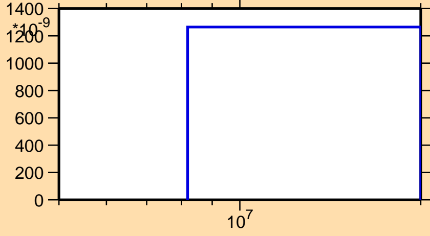
\sigma vs. E for ^{129}\text{Ce}(n,\text{pd})
