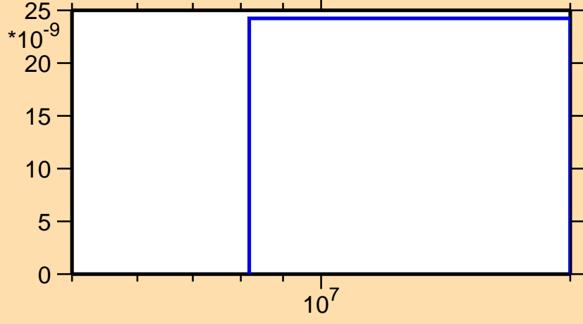
\sigma vs. E for ^{129}\text{Ce}(n,\text{pt})
