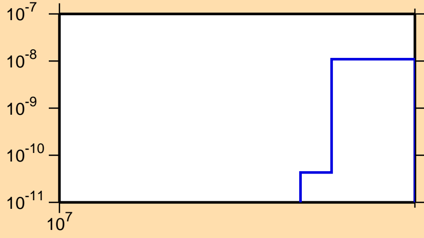
\sigma vs. E for ^{130}\text{Ce}(n,2n\alpha)
