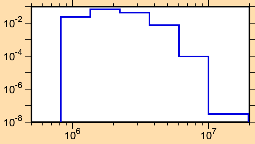
\sigma vs. E for ^{130}\text{Ce}(n,n_4)
