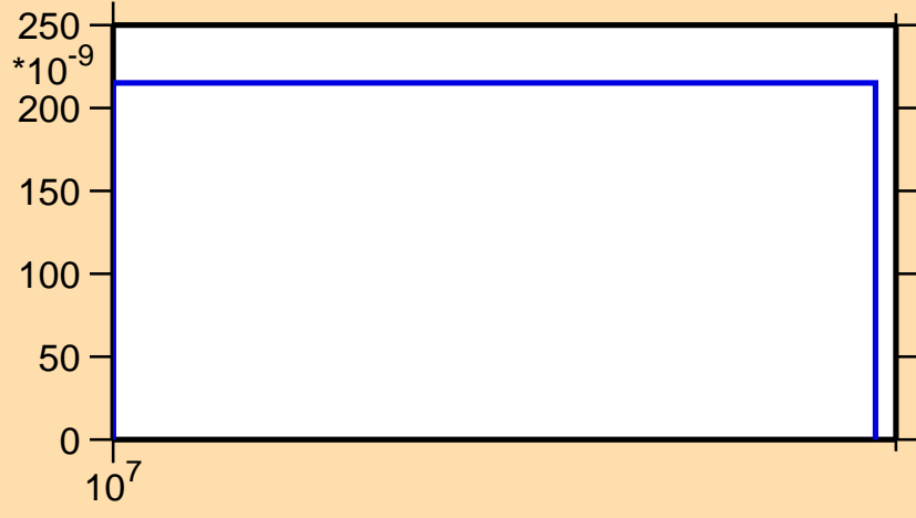
\sigma vs. E for ^{130}\text{Ce}(n,\text{pd})
