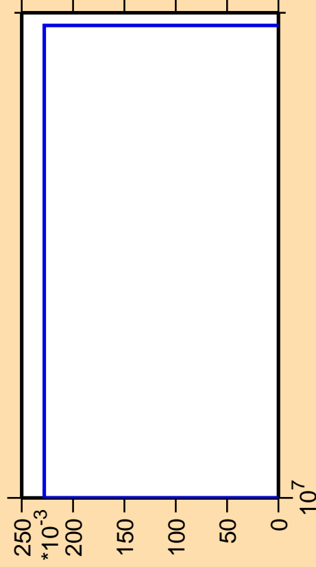
\Delta\sigma/\sigma vs. E for ^{130}\text{Ce} (mt 34)
