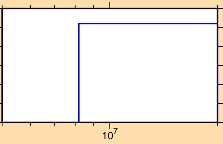
\sigma vs. E for ^{130}\text{Ce}(\text{mt } 45)
