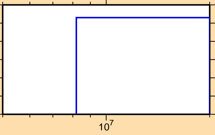
\sigma vs. E for ^{131}\text{Ce}(n,2np)
