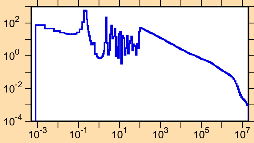
\sigma vs. E for ^{131}\text{Ce}(n,\gamma)
