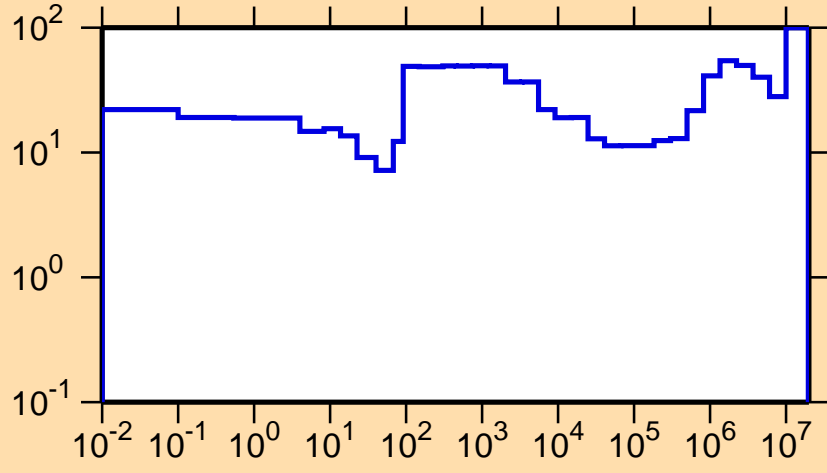
\Delta\sigma/\sigma vs. E for ^{131}\text{Ce}(n,\gamma)
