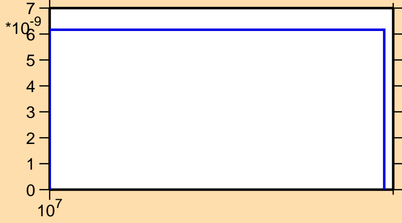
\sigma vs. E for ^{131}\text{Ce}(n,\text{pt})
