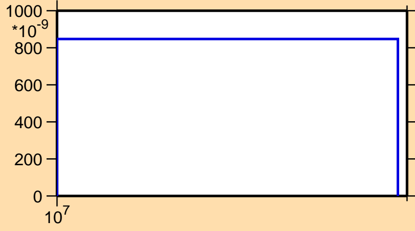
\sigma vs. E for ^{131}\text{Ce}(n,2n\alpha)
