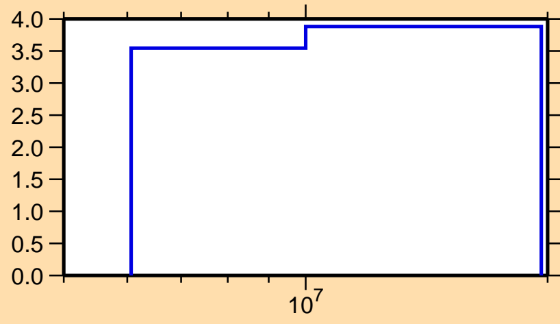
\Delta\sigma/\sigma vs. E for ^{131}\text{Ce}(n,\text{nonel.})
