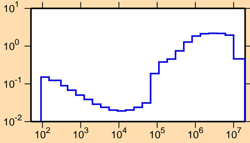
\sigma vs. E for ^{131}\text{Ce}(n,\text{inel.})
