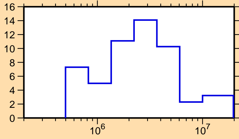
\Delta\sigma/\sigma vs. E for ^{131}\text{Ce}(n,\text{el.})
