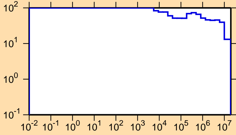
\Delta\sigma/\sigma vs. E for ^{131}\text{Ce}(n,p)
