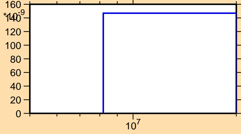
\sigma vs. E for ^{131}\text{Ce}(n,\text{pd})
