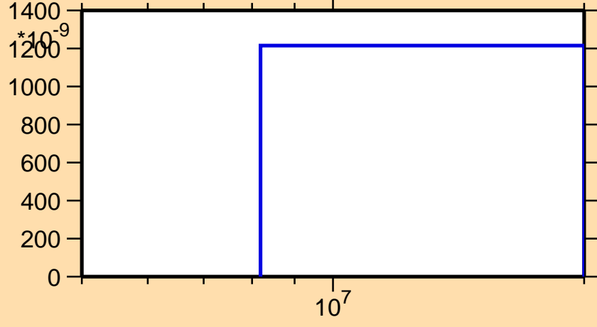
\sigma vs. E for ^{131}\text{Ce}(n,\text{He3})
