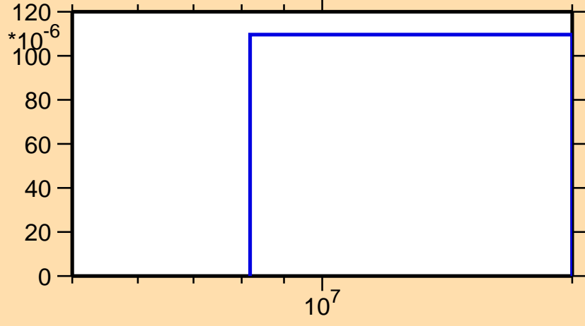
\sigma vs. E for ^{131}\text{Ce}(n,t)
