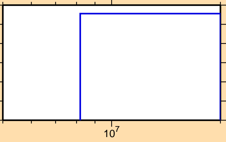
\sigma vs. E for ^{131}\text{Ce}(n,\text{pt})
