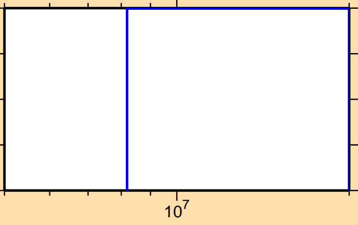
\sigma vs. E for ^{131}\text{Ce}(\text{mt117})
