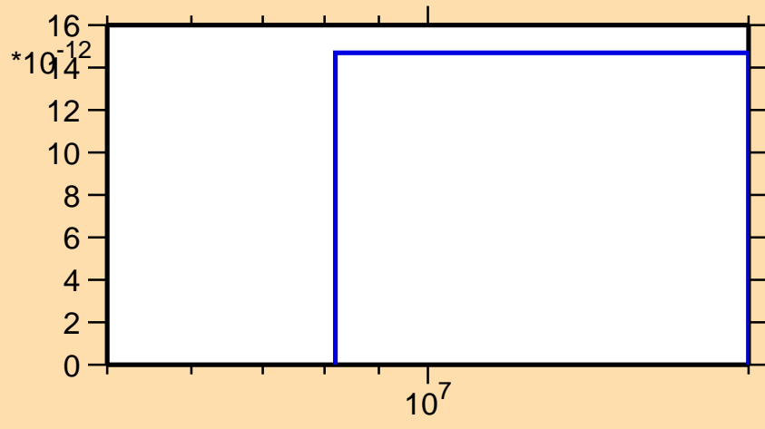
\sigma vs. E for ^{131}\text{Ce}(\text{mt } 34)
