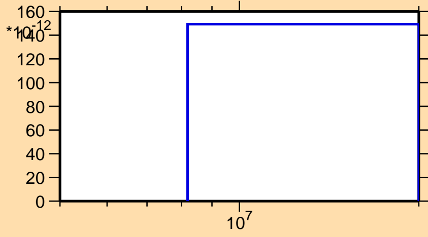
\sigma vs. E for ^{131}\text{Ce} (mt 45)
