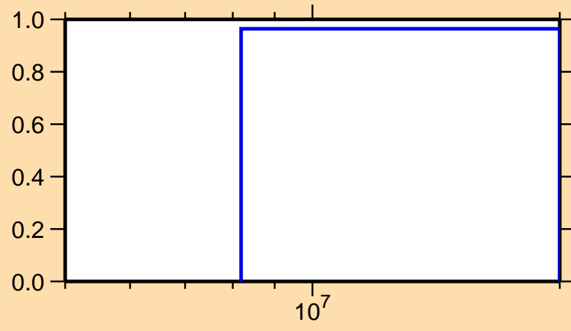
\sigma vs. E for ^{131}\text{Ce}(n,2n)
