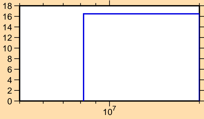
\Delta\sigma/\sigma vs. E for ^{131}\text{Ce}(n,2n)
