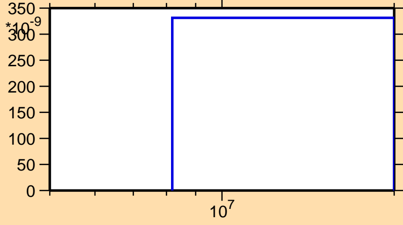
\sigma vs. E for ^{131}\text{Ce}(n,\text{nd})
