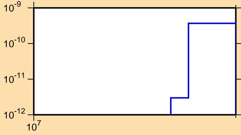
\sigma vs. E for ^{132}\text{Ce} (mt 45)
