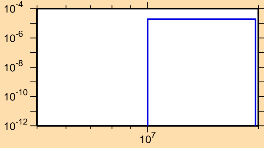
\sigma vs. E for ^{132}\text{Ce}(n,t)
