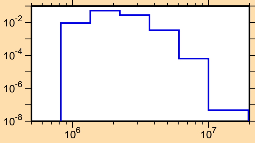
\sigma vs. E for ^{132}\text{Ce}(n,n_4)
