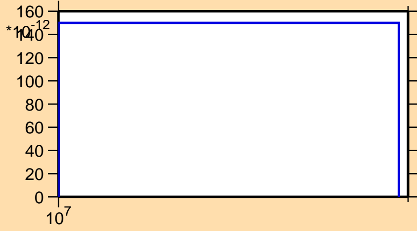
\sigma vs. E for ^{132}\text{Ce}(n,2np)
