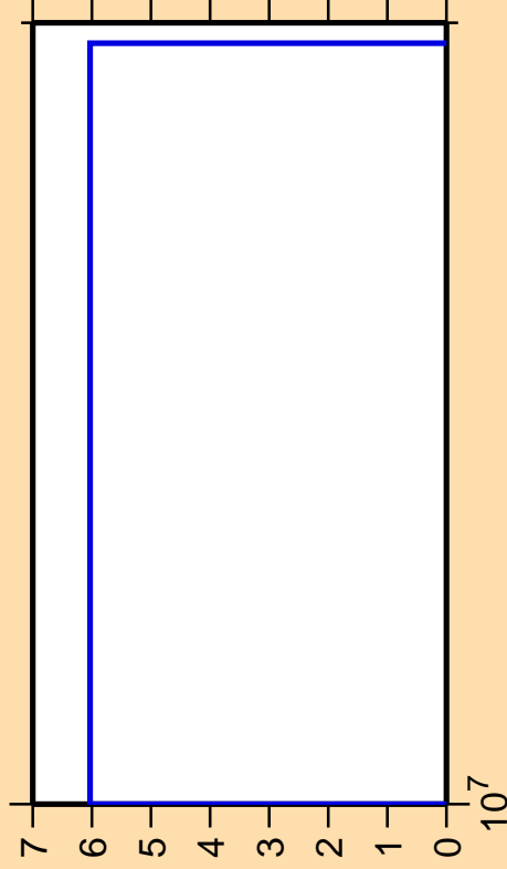
\Delta\sigma/\sigma vs. E for ^{132}\text{Ce} (mt 45)
